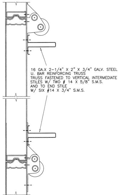
INTERMEDIATE SECTIONS REINFORCING
