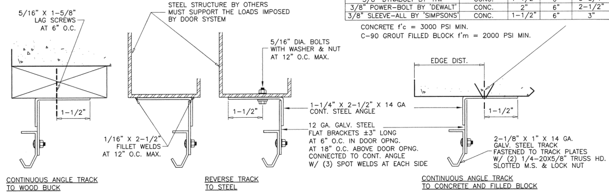
ALTERNATE TRACK INSTALLATION
