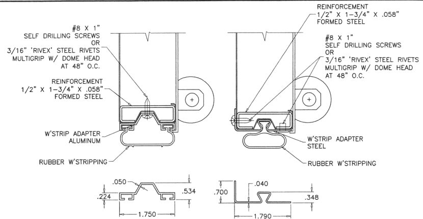
BOTTOM SEAL OPTIONS
