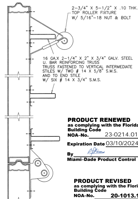
TOP SECTION REINFORCING
