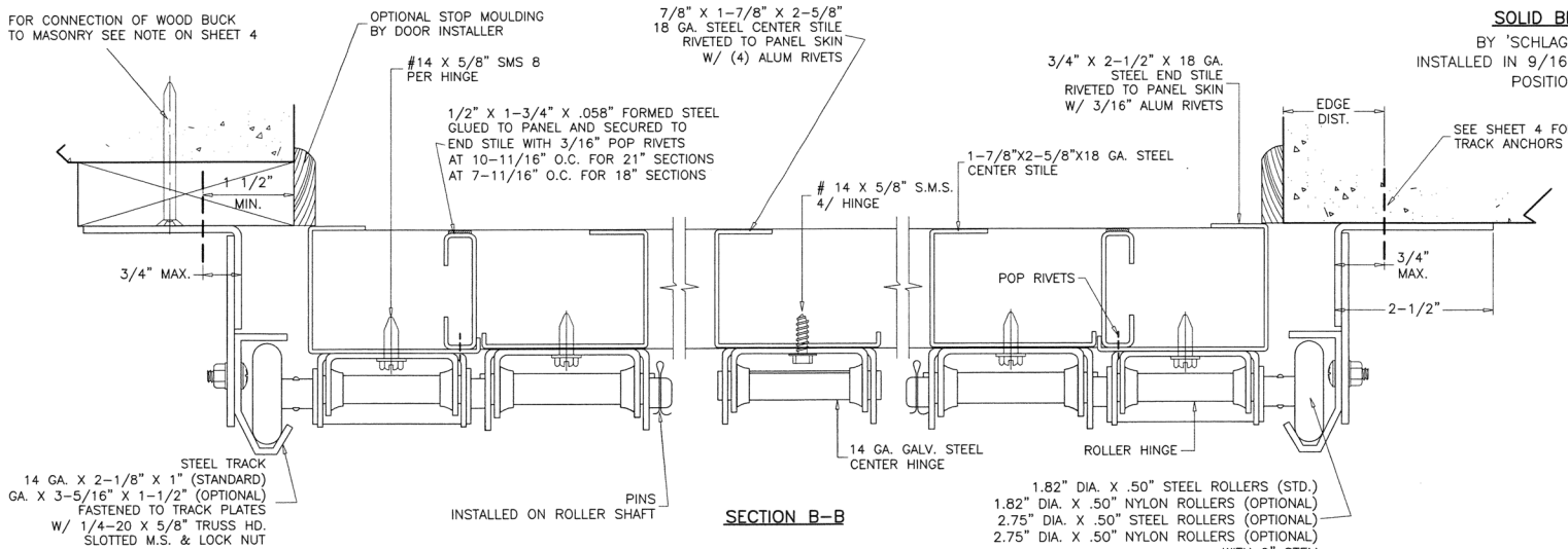
1ST SECTION (BOTTOM) REINFORCING
