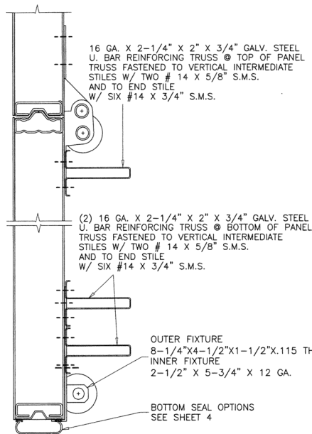
1ST SECTION (BOTTOM) REINFORCING
