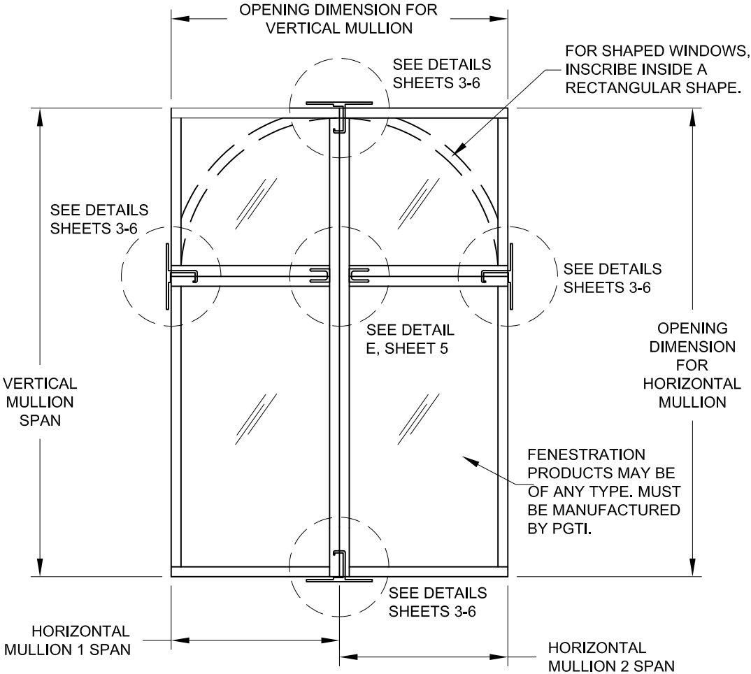
FIGURE 1: MULTIPLE MULLIONS
