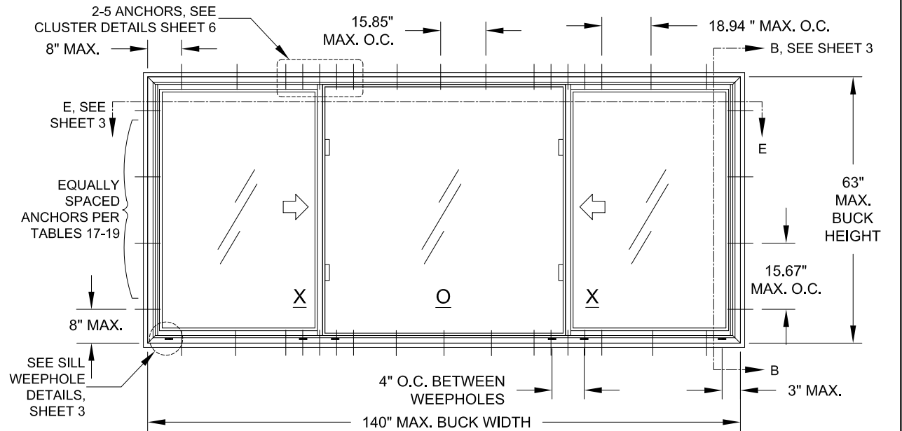
ELEVATION FOR TYP. FLANGE FRAME SHOWN AS XO configuration
