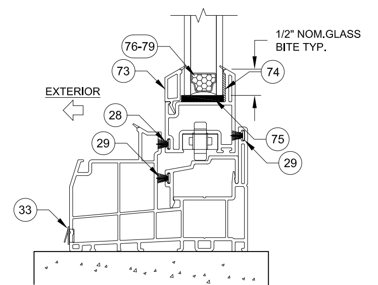
TYP. GLAZING DETAIL
