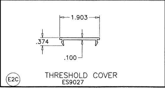
E2D MEDIUM THRESHOLD NOT APPR'D FOR WATER RESISTANCE
