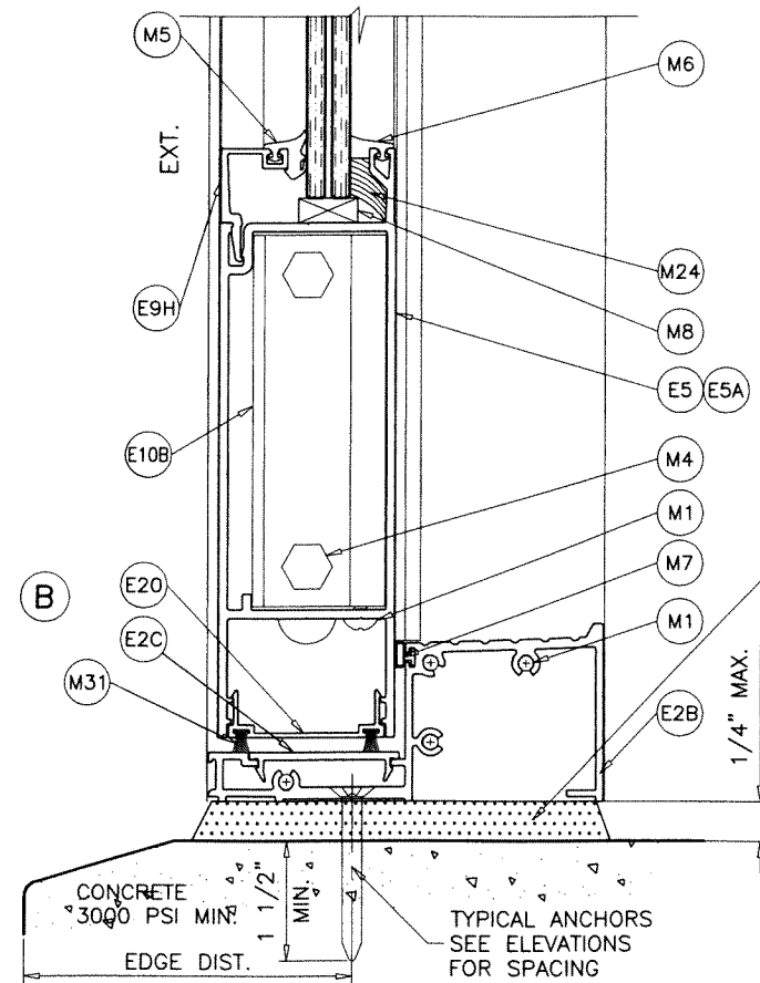
HIGH THRESHOLD APPROVED FOR WATER RESISTANCE WHEN USED WITH SINGLE DOORS (SEE SHEET 2) NOT APPROVED FOR WATER RESISTANCE WHEN USED WITH DOUBLE DOORS
