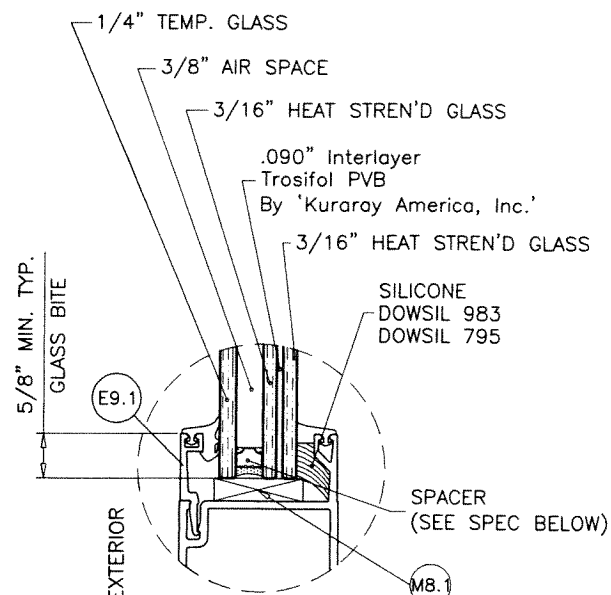
GLASS TYPE 'C' 1-1/8" OVERALL INSUL. LAM. GLASS
