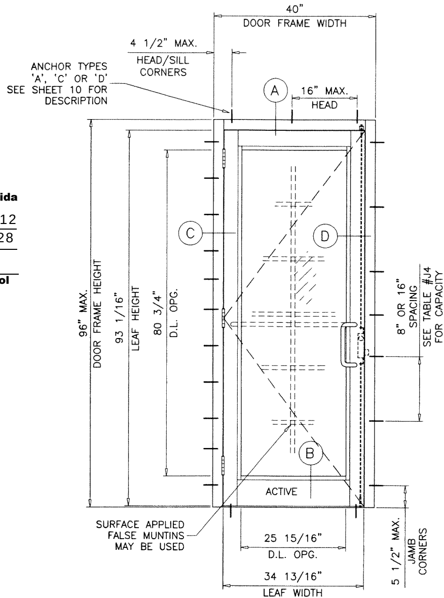
TYPICAL ELEVATION (X)
