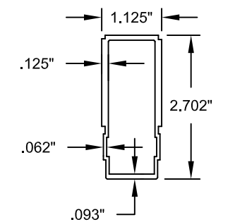
71 FRAME ASSEMBLY TUBE #7004, 6063-T6
