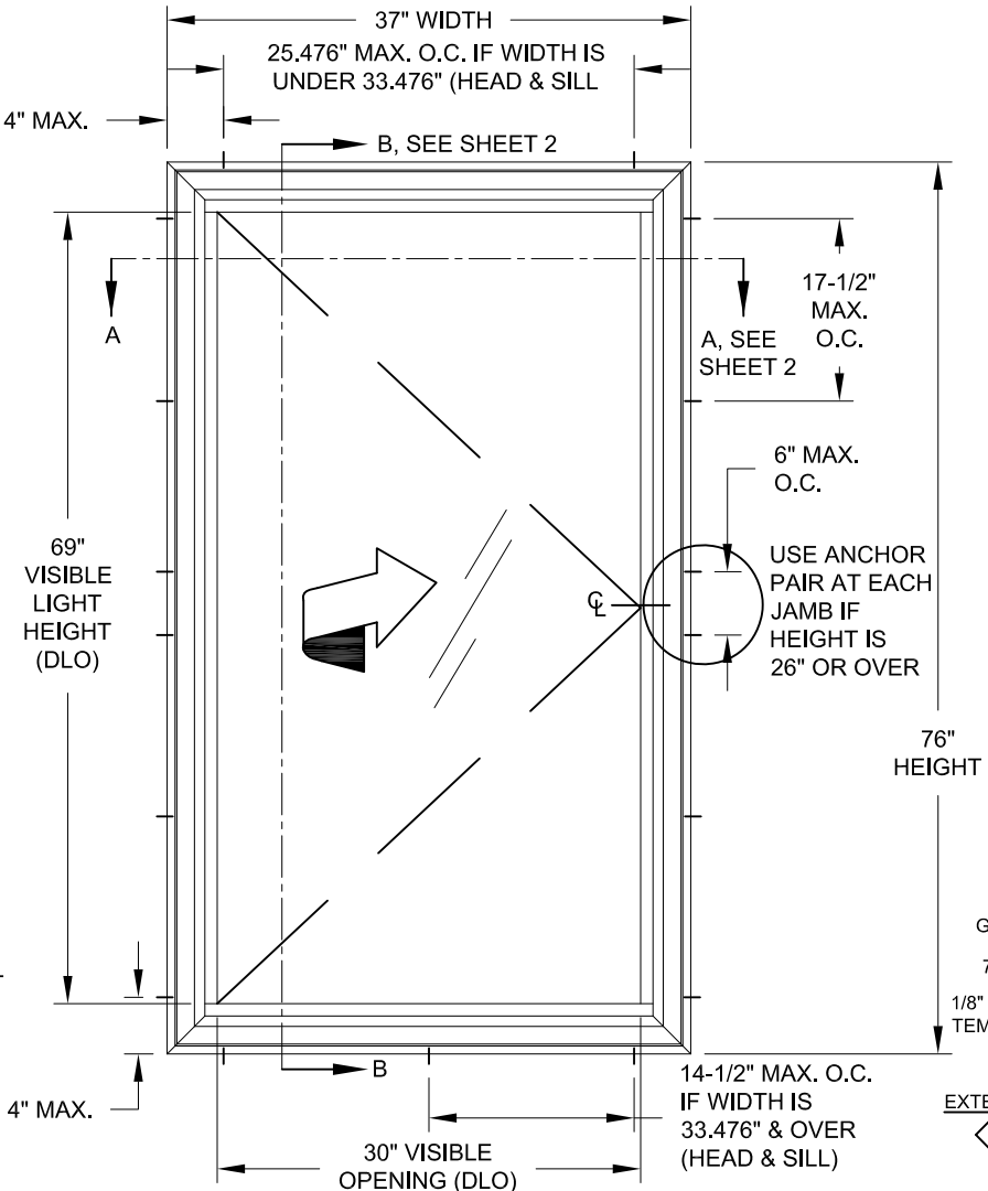
TYP. ELEVATION OF CASEMENT WINDOW
