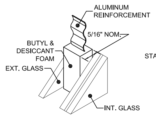
102 DURASEAL® SPACER
