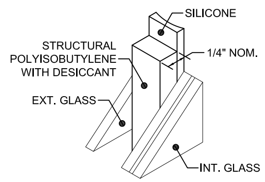
100 KODISPACE 4SG TPS
