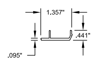
2 ANCHOR PLATE #7071, 6063-T6
