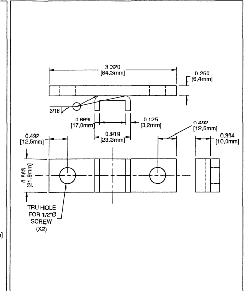
⑩ WALL ATTACHMENT END CAP EC01WC-V1 SS304/SS316
