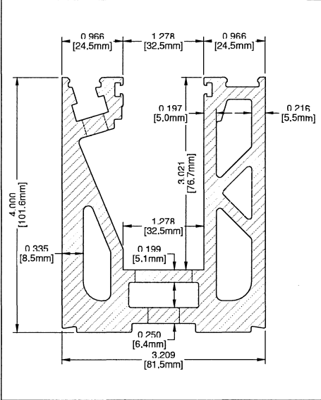
① BASE SHOE 144" LONG SE-76.2TD-V1 ALUM-6063-T6
