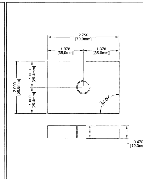
⑨ WELD BLOCK WP115SH-V1 SS304/SS316
