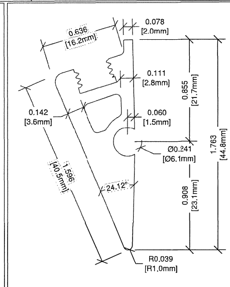
② SUPPORT ARM 144" LONG SE-ARM200-V1 ALUM-6063-T6
