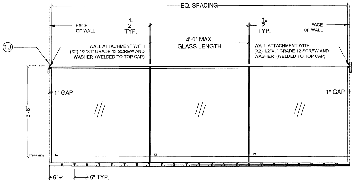
3/4" LAMINATED GLASS WELDED
