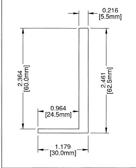
⑤ 'L' SHIM 4" LONG SE-LS19 NYLON
