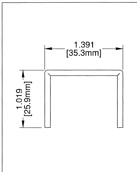
14 'U' CAP 144" LONG CR121DC SS304/SS316
