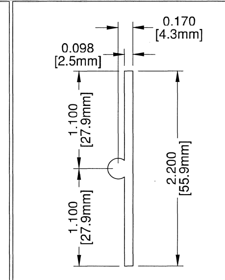
11 SWIVEL GASKET 144" LONG SE-GA25 NYLON
