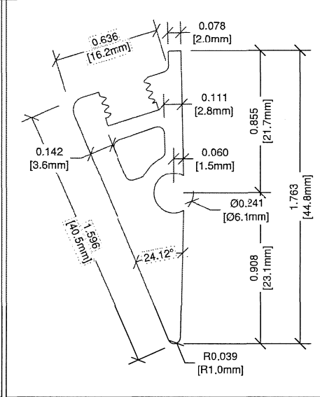
② SUPPORT ARM 144" LONG SE-ARM200-V1 ALUM-6063-T6
