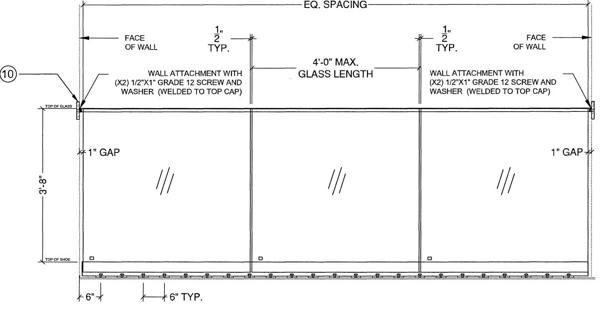
1" LAMINATED GLASS WELDED
