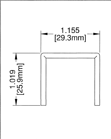
⑦ 'U' CAP 144" LONG CR120DC SS304/SS316
