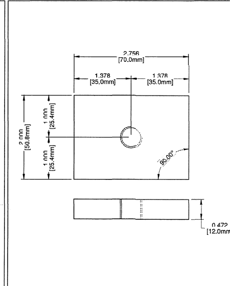
⑨ WELD BLOCK WP115SH-V1 SS304/SS316
