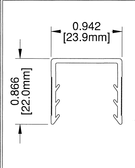
⑧ 'U' CAP GASKET GAEP120U EPDM
