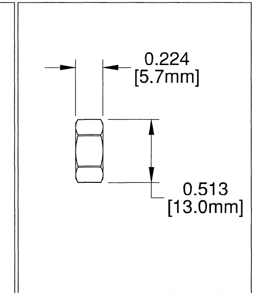
17 M8 NUT FM8NUT SS304/SS316
