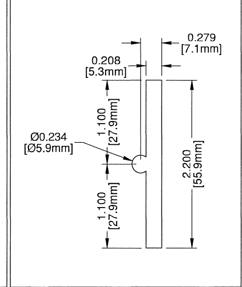
④ SWIVEL GASKET 144" LONG SE-GA19 NYLON
