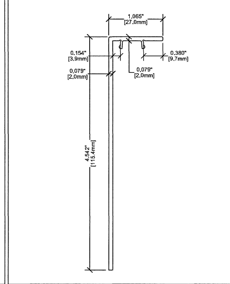
③ ALUMINUM EXTRUDED CLADDING CL800LO ALUM-6063-T6
