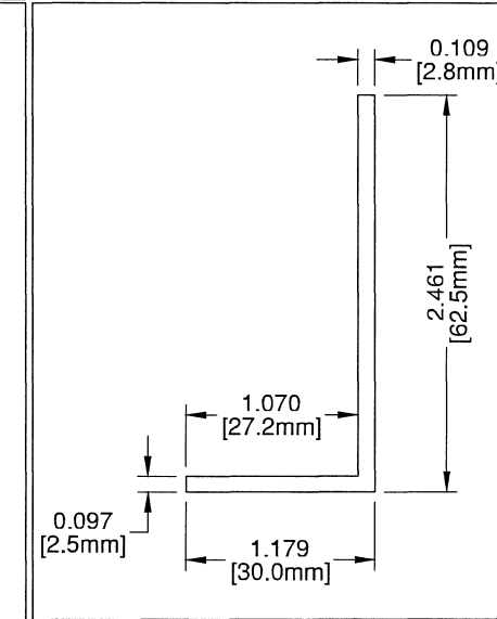
12 'L' SHIM 4" LONG SE-LS25 NYLON
