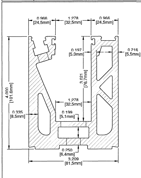
① BASE SHOE 144" LONG SE-76.2TD-V1 ALUM-6063-T6
