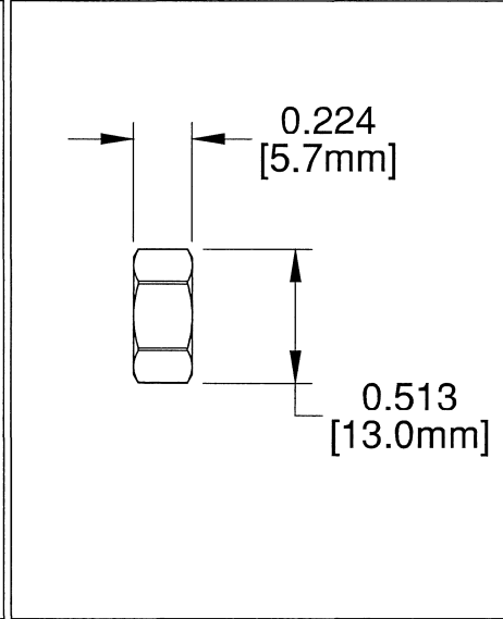
⑪ M8 NUT FM8NUT SS304/SS316
