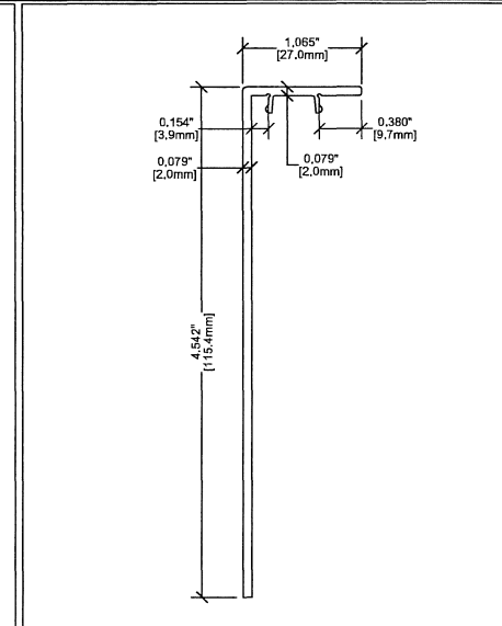
③ ALUMINUM EXTRUDED CLADDING CL800LO ALUM-6063-T6
