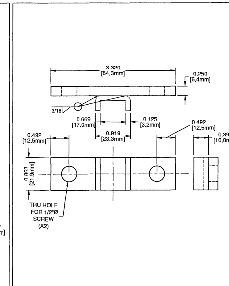
10 WALL ATTACHMENT END CAP EC01WC-V1 SS304/SS316
