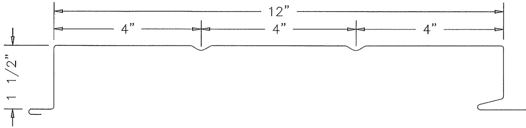
TYPICAL PANEL PROFILE
