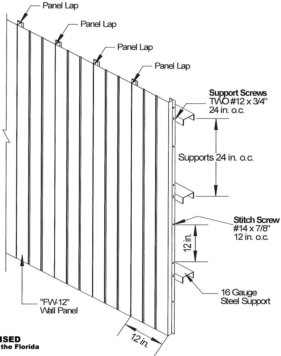
TYPICAL ELEVATION VIEW OUTSIDE OF WALL ASSEMBLY
