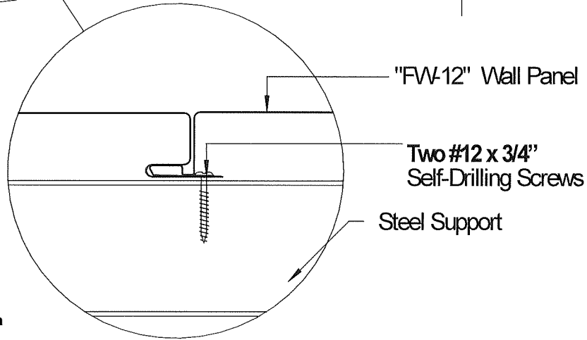
TYPICAL PANEL ASSEMBLY SECTION VIEW
