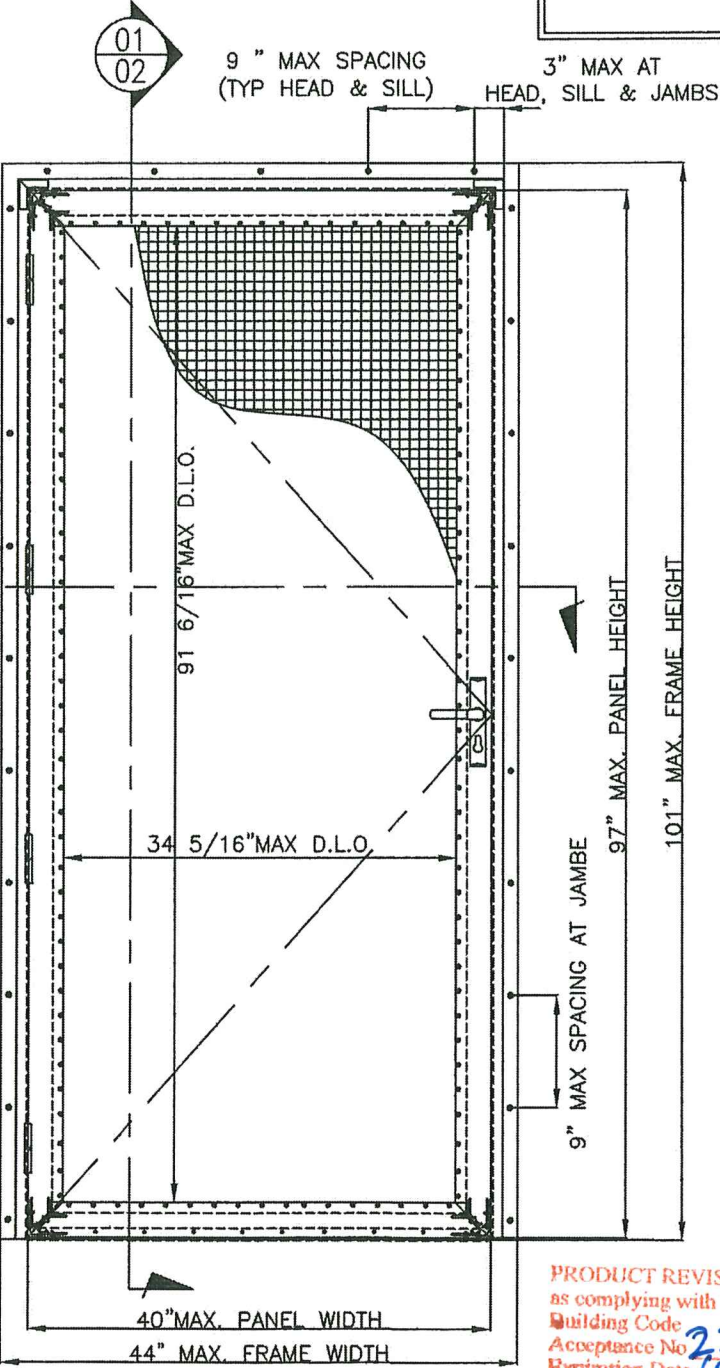
01 01 TYPICAL ELEVATION SCALE EXTER ELEV
