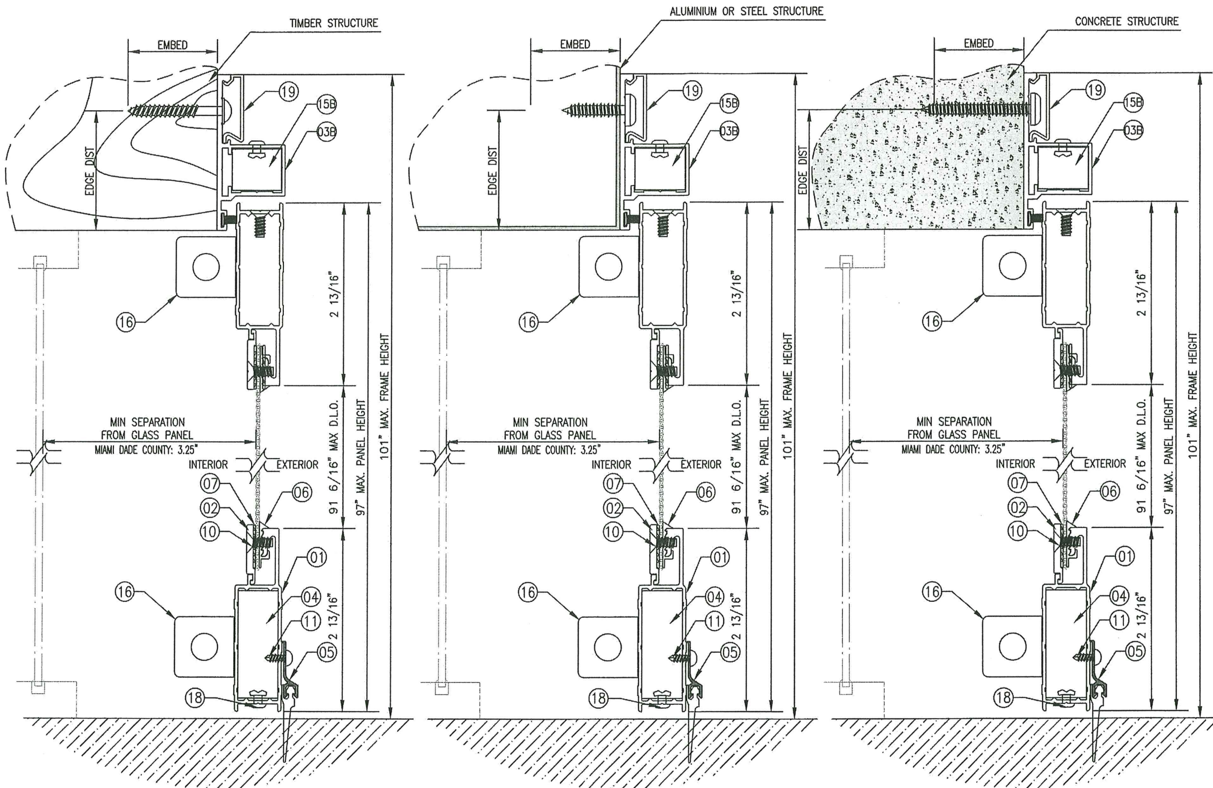
ATTACHMENT TO WOOD
