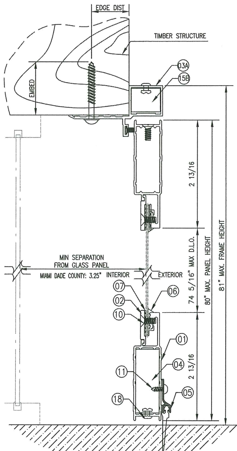
ATTACHMENT TO WOOD
