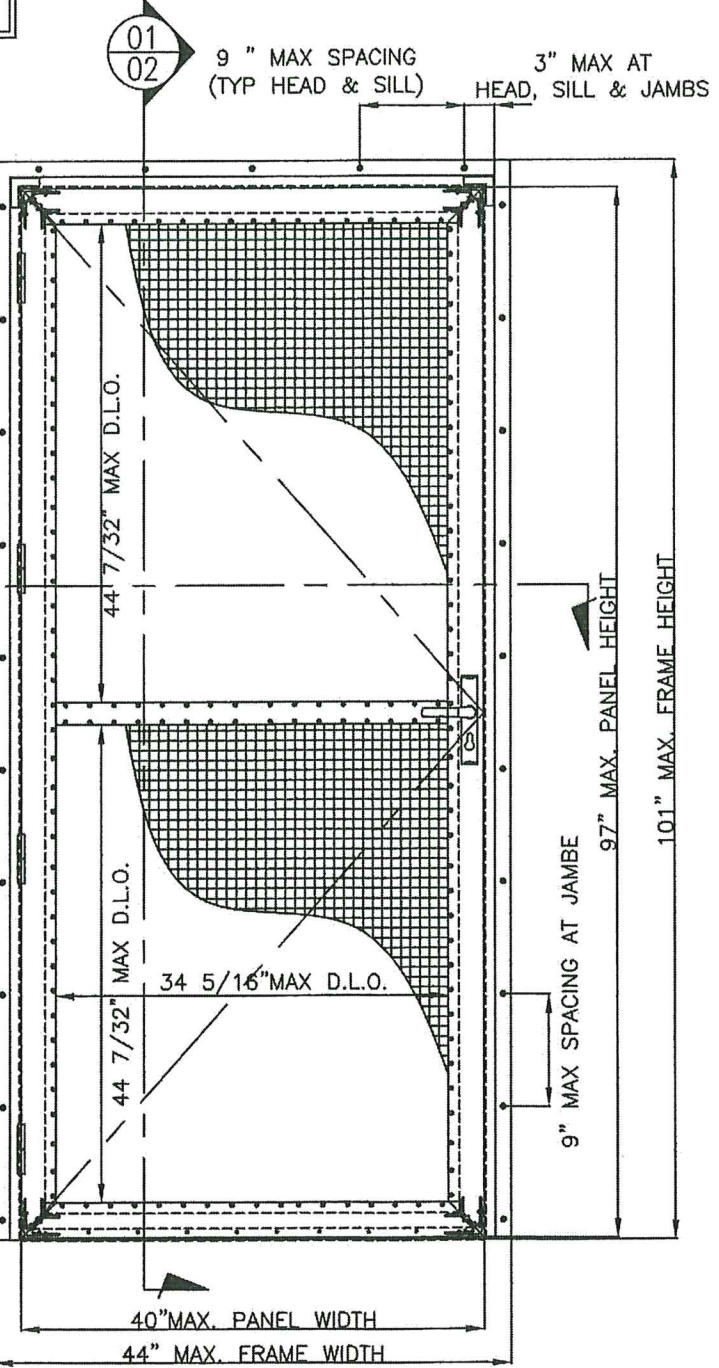
01 01 TYPICAL ELEVATION WITH MIDRAIL SCALE EXTER ELEV
