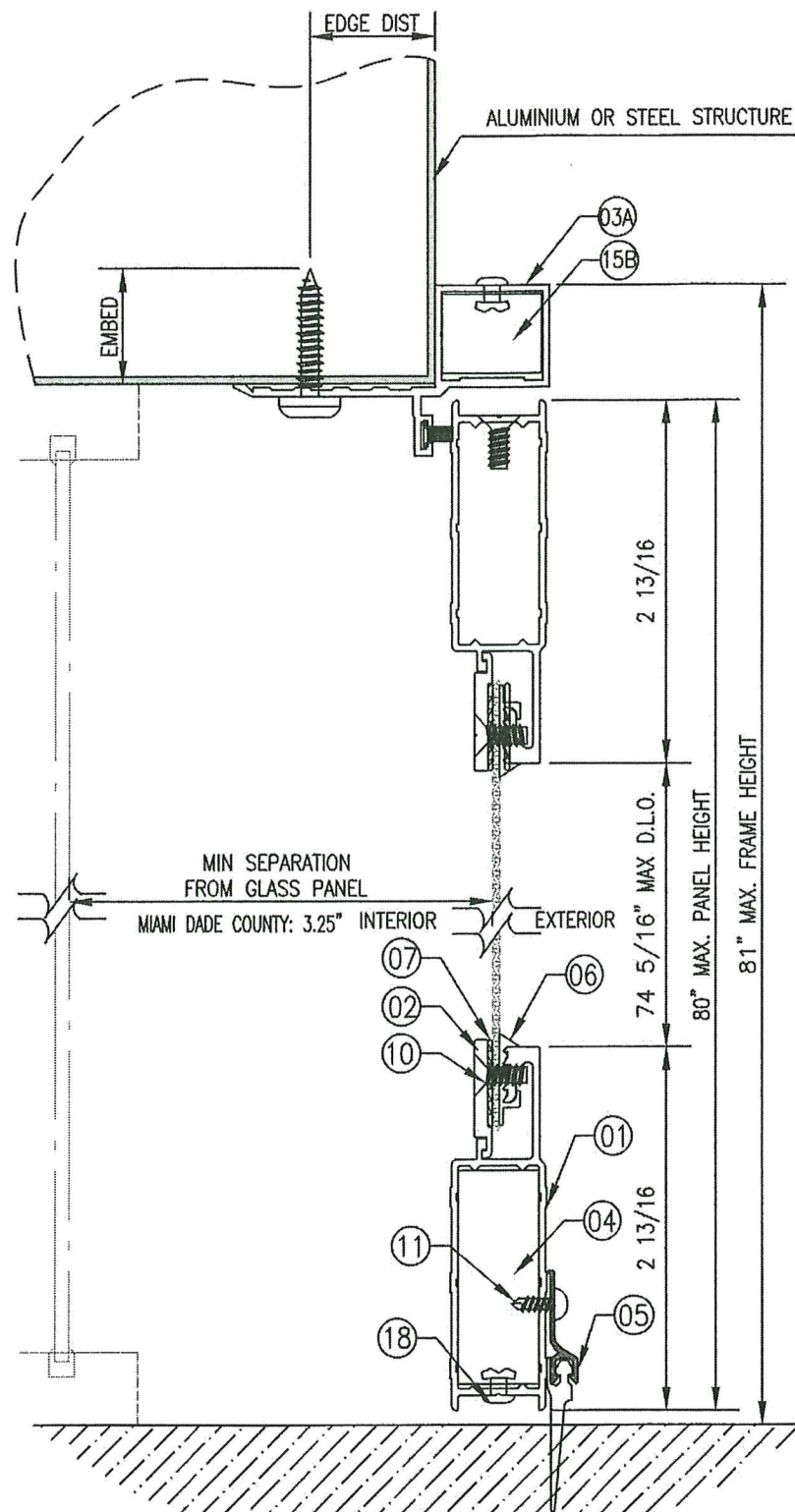
ATTACHMENT TO ALUMINIUM OR STEEL
