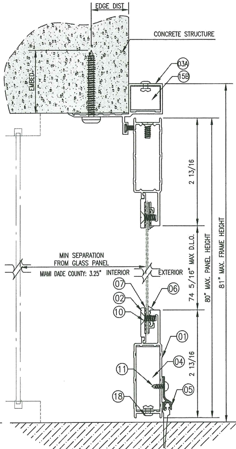
ATTACHMENT TO HOLLOW BLOCK OR CONCRETE
