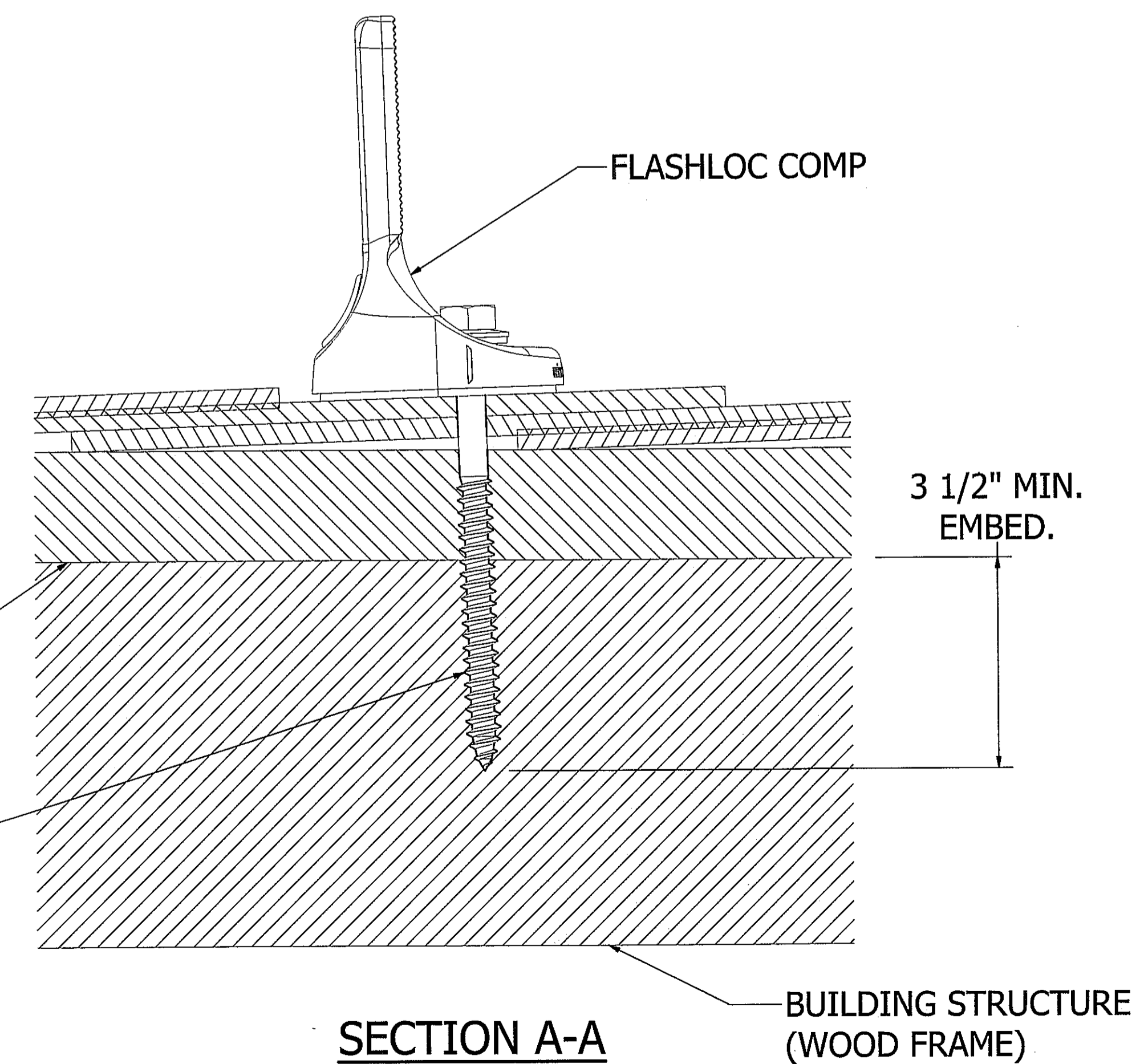
SECTION FLASHLOC COMP DETAIL NOT TO SCALE
