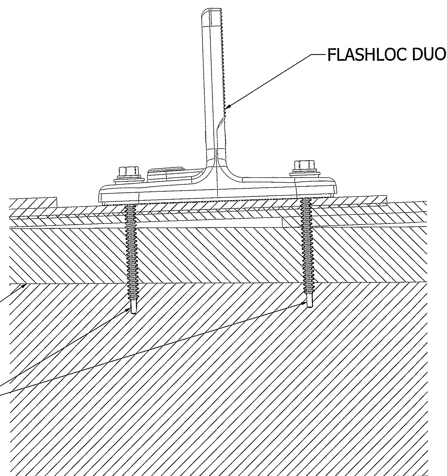
SECTION FLASHLOC DUO DETAIL NOT TO SCALE
