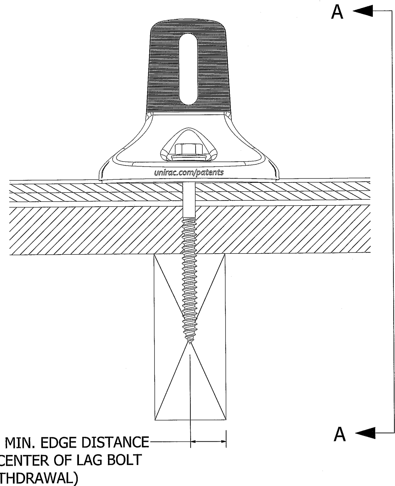
SECTION FLASHLOC COMP DETAIL NOT TO SCALE
