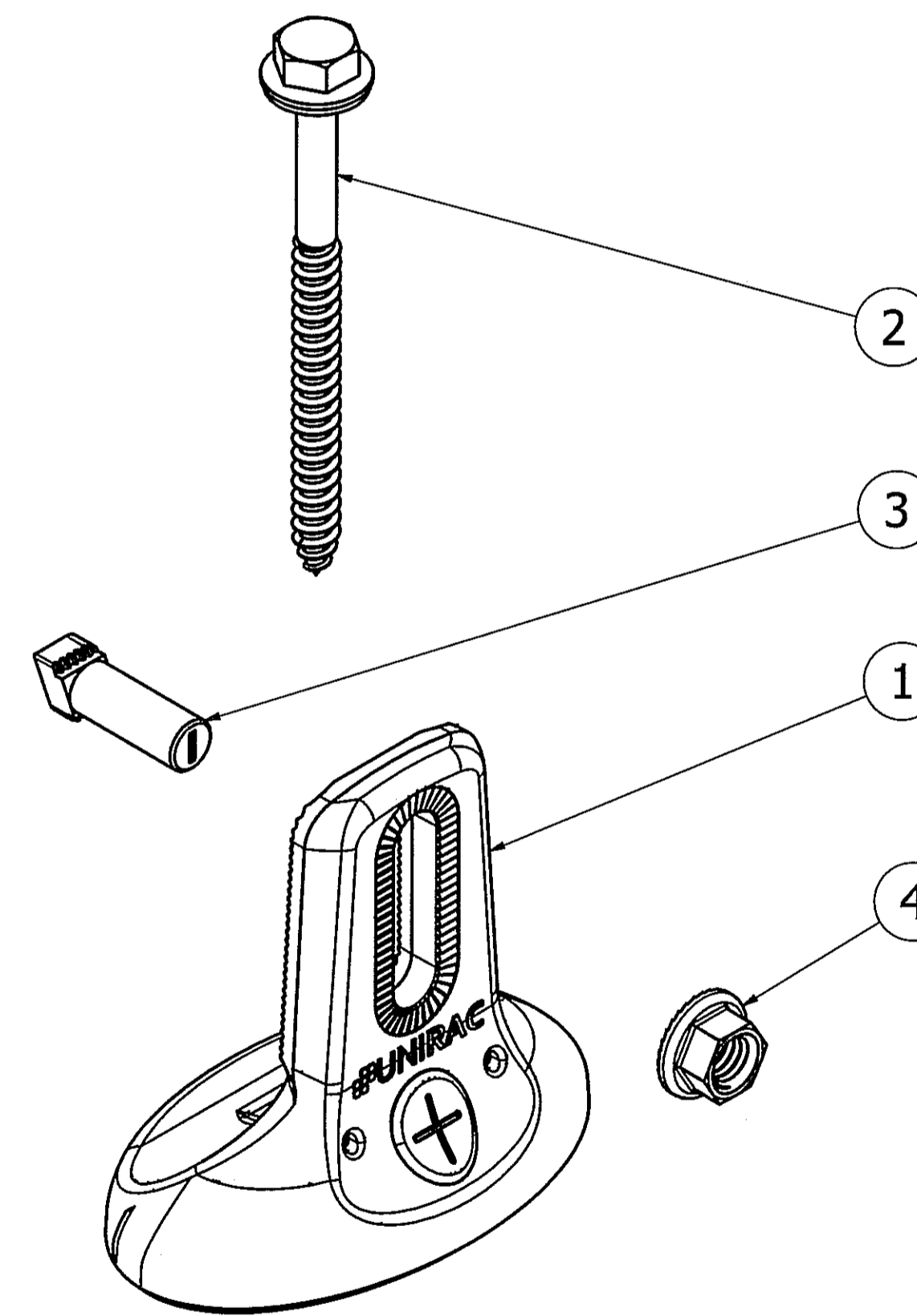
EXPLODED VIEW
