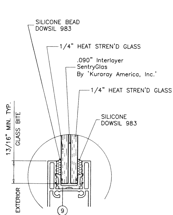
GLASS TYPE 'A' 9/16" OVERALL LAM. GLASS
