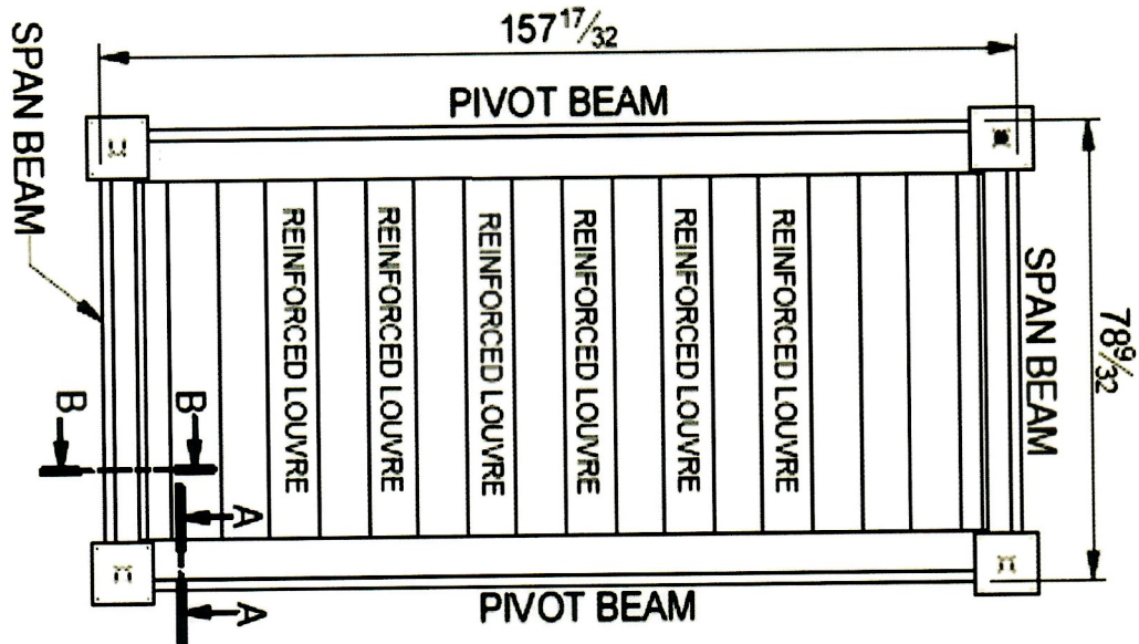
CAMARGUE - PERGOLA 3 TOP VIEW
