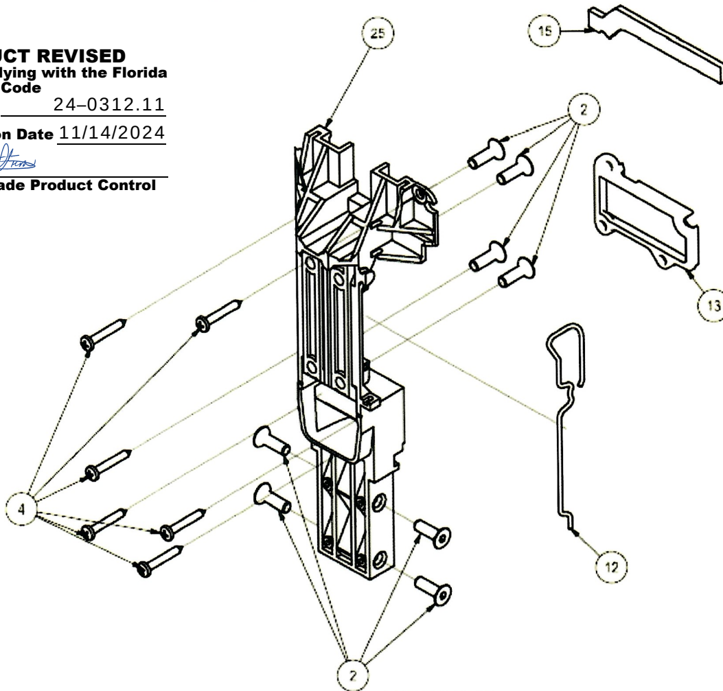
DETAIL: A (1:3)
