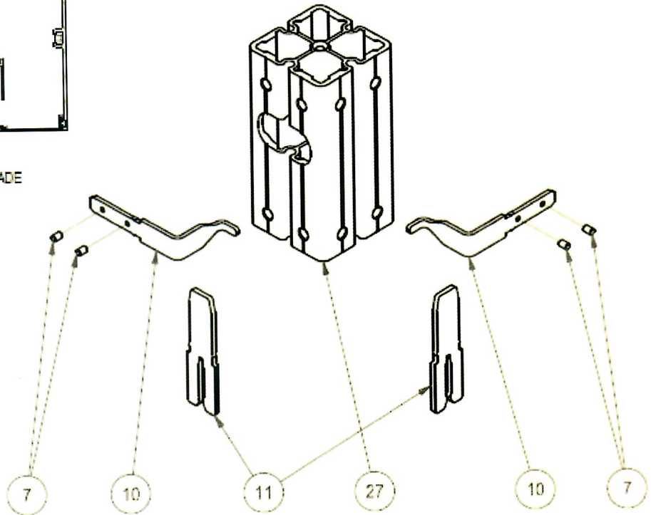
DETAIL: C (1:3)
