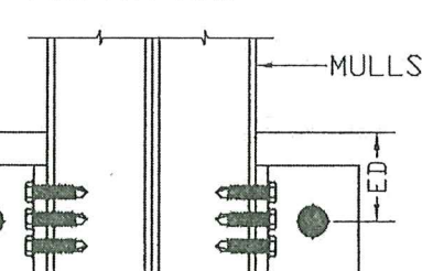
CONNECTION 11.6 DUAL MULLIONS TWO ANCHORS
