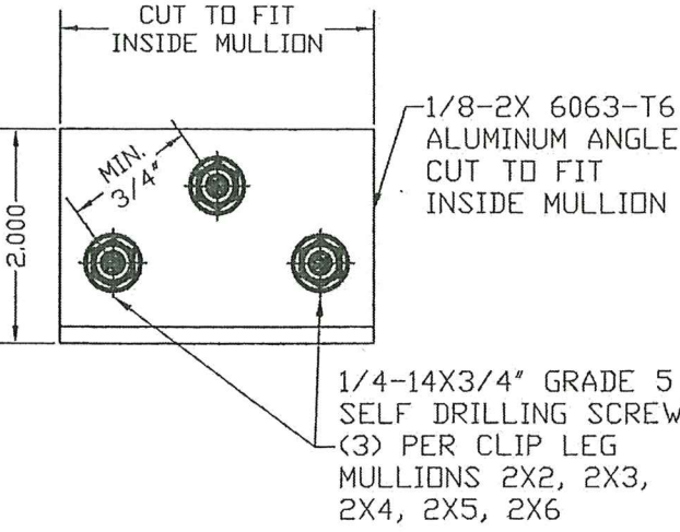
CONNECTION 9 CLIP ANCHORED TO MULLION BAR
