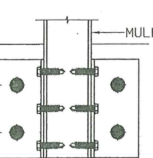
CONNECTION 11.4 SINGLE MULLION FOUR ANCHORS
