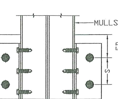
CONNECTION 11.7 DUAL MULLIONS FOUR ANCHORS
