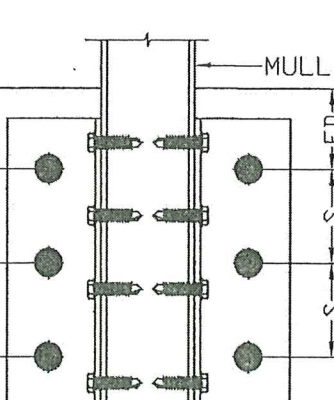
CONNECTION 11.5 SINGLE MULLION SIX ANCHORS
