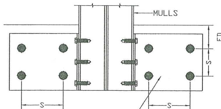
CONNECTION 11.9 DUAL MULLIONS EIGHT ANCHORS
