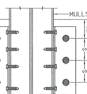
CONNECTION 11.8 DUAL MULLIONS SIX ANCHORS
