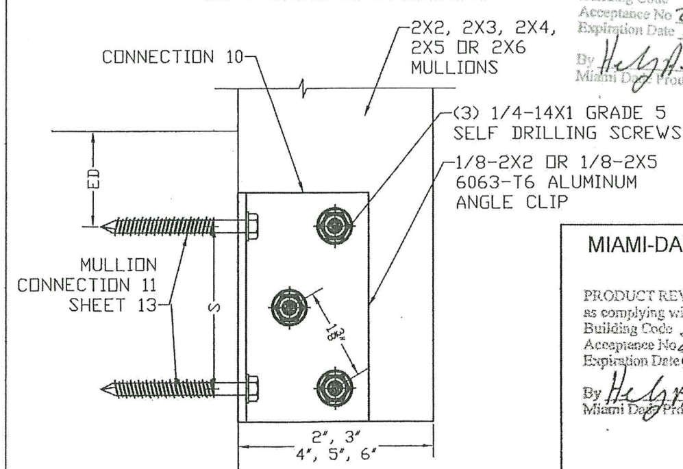
CONNECTION 10 CLIP ANCHORED TO MULLION BAR
