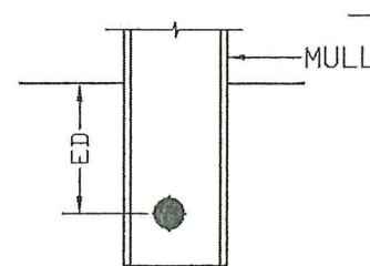
CONNECTION 11.1 SINGLE MULLION ONE ANCHOR
