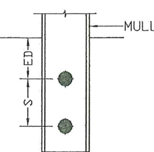
CONNECTION 11.2 SINGLE MULLION TWO ANCHORS
