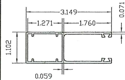
1- TRACK TYPE A 6063-T6 ALLOY (min. Fty= 23.1 Ksi)
