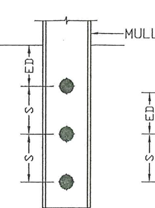
CONNECTION 11.3 SINGLE MULLION THREE ANCHORS
