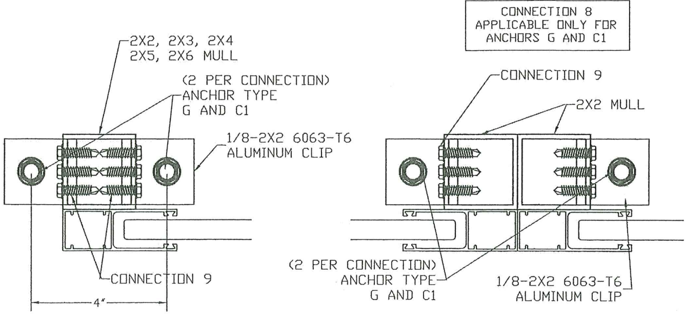
CONNECTION 8 FLOOR/CEILING MOUNTED TO CONCRETE
