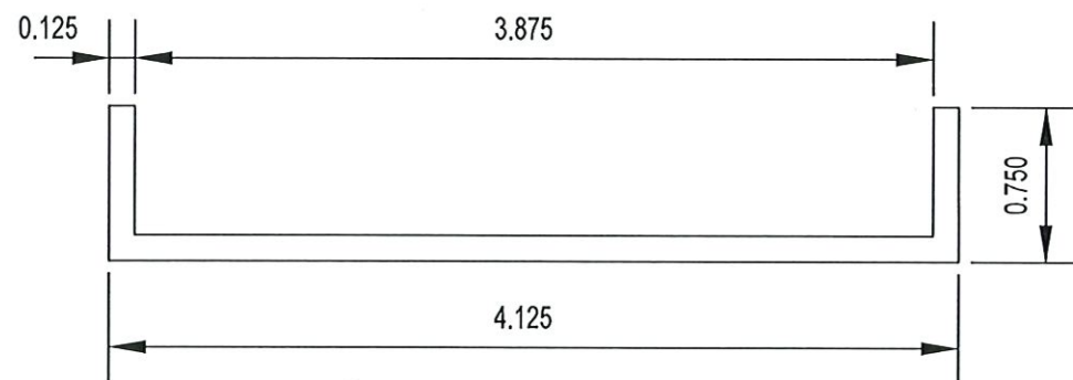
PVC CHANNEL SCALE 1:1
