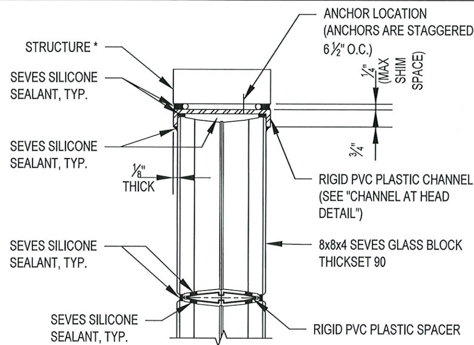
TYPICAL HEAD DETAIL SCALE: 3" = 1'-0"
