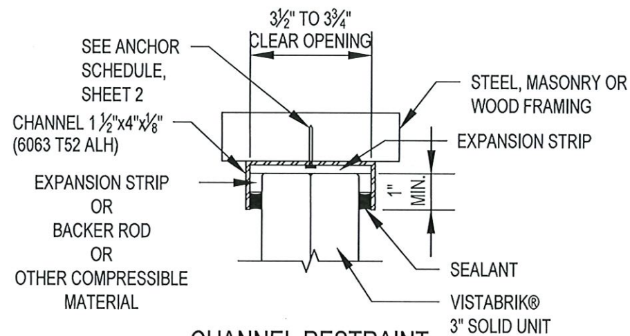
CHANNEL RESTRAINT DETAIL
