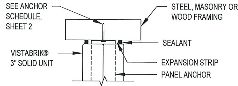
PANEL ANCHOR RESTRAINT DETAIL
