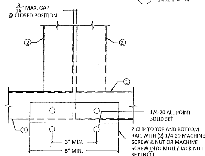
L CLOSURE ANGLE (TYPICAL TOP & BOTTOM AT CENTER JOINT)
