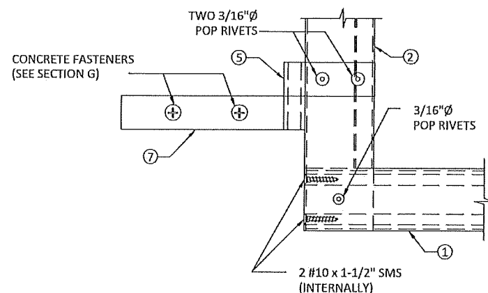
K TYPICAL SIDE RAIL TO TOP & BOTTOM RAIL CONNECTION
