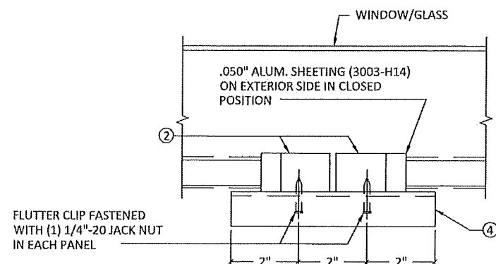
D SHEETING & FLUTTER CLIP DETAIL
