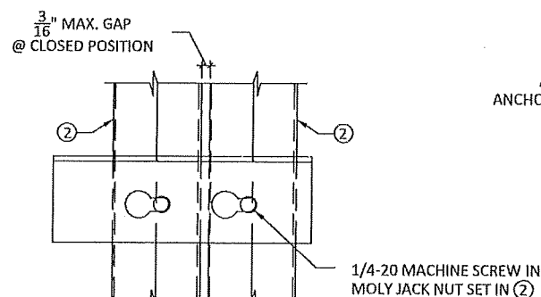
N FLUTTER CLIP DETAIL
