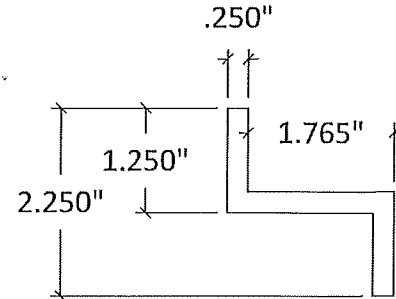
3 Z-BRACKET HALF SCALE
