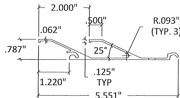
12 IMPACT RESISTANT STANDARD 2 LOUVER BLADE HALF SCALE
