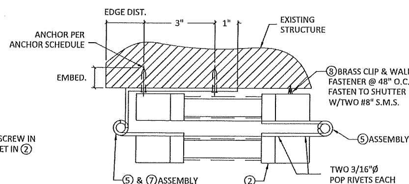
P DOUBLE UNIT HINGE ASSEMBLY DETAIL
