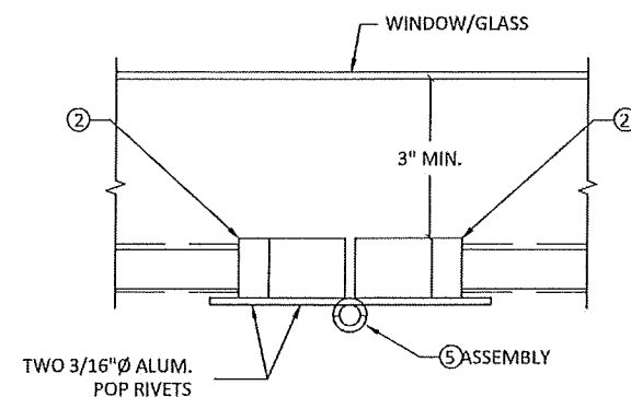
E "A" HINGE ASSEMBLY DETAIL
