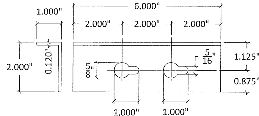
4 FLUTTER CLIP HALF SCALE
