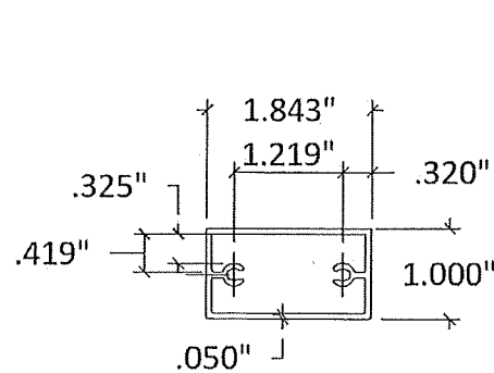
1 TOP & BOTTOM RAIL HALF SCALE
