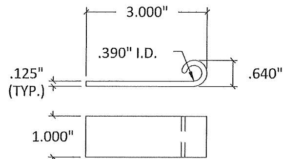
5 "A" HINGE HALF SCALE
