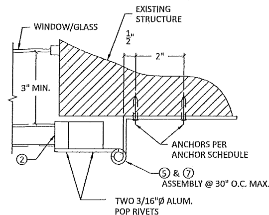
F "C" HINGE ASSEMBLY DETAIL
