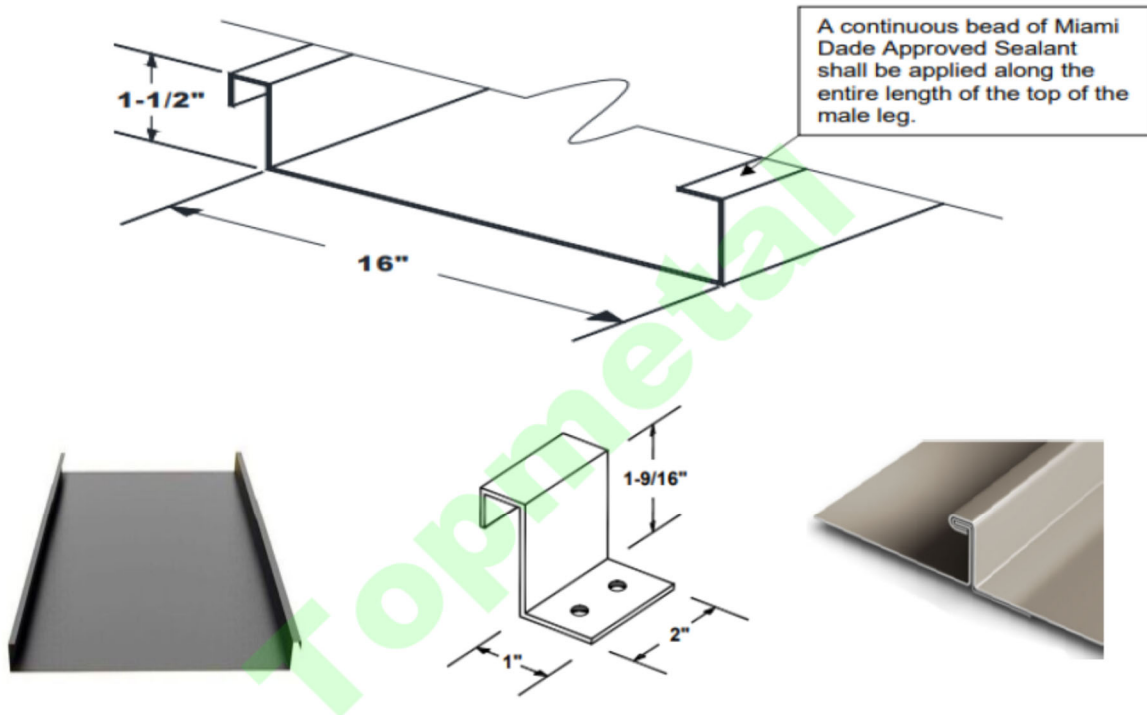
Panel Detail
