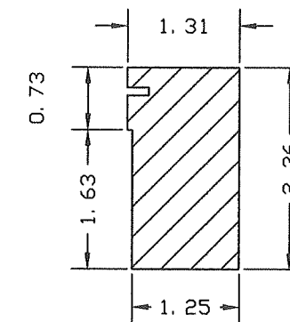
11- THRESHOLD CAP
