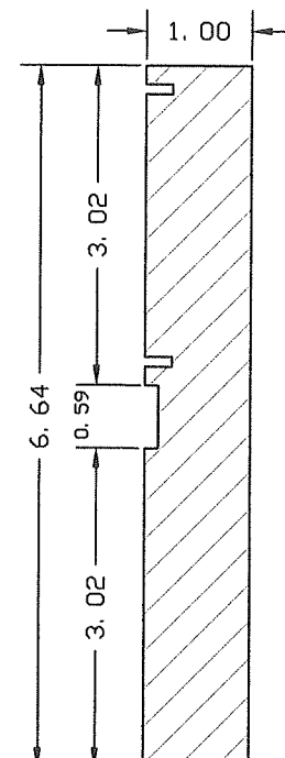
9B- SIDE JAMB WEIGHT & CHAIN
