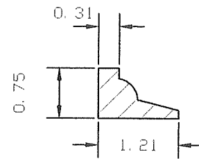
6- INTERIOR GLASS STOP FOR USE WITH GLASS OPTION A
