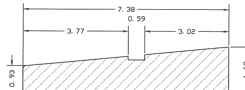
10- THRESHOLD
