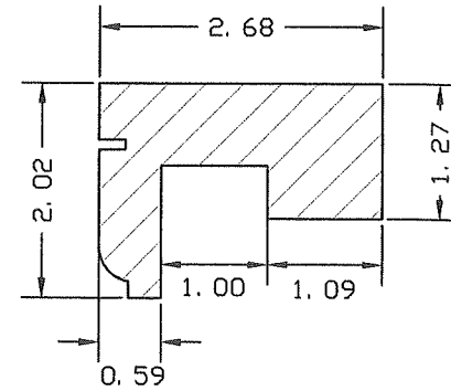
3- TOP RAIL ACTIVE SLAB
