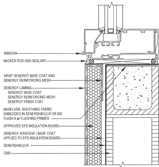
TYPICAL WINDOW SILL FLUSH
