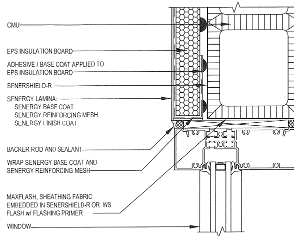
TYPICAL WINDOW JAMB (FLUSH)
