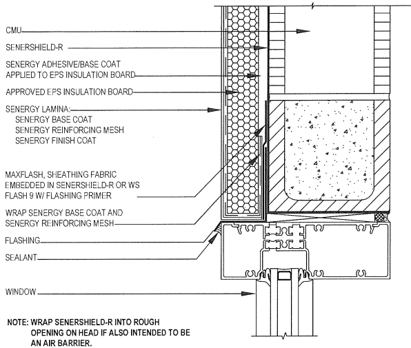
TYPICAL WINDOW HEAD (FLUSH)
