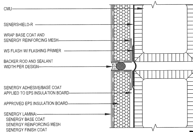
TYPICAL EXPANSION JOINT (PLAN VIEW)
