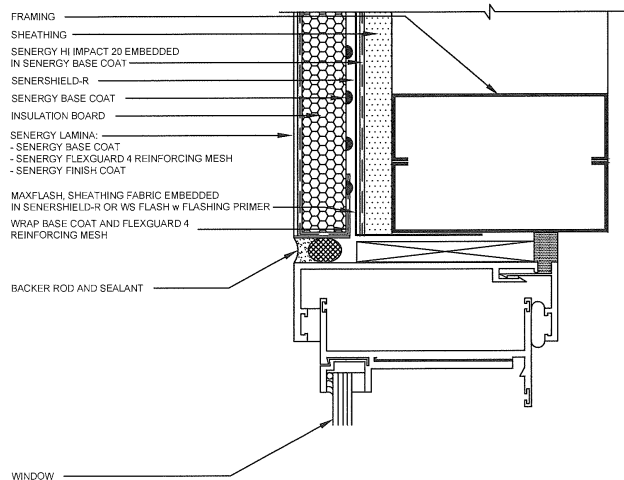
WINDOW JAMB DETAIL (FLUSH)
