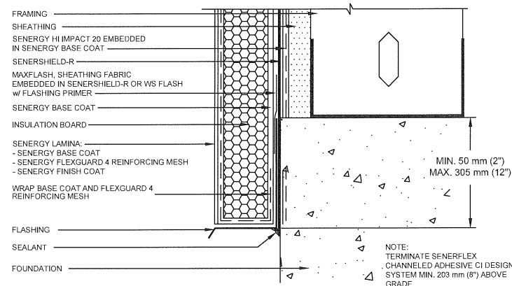
TERMINATION AT FOUNDATION
