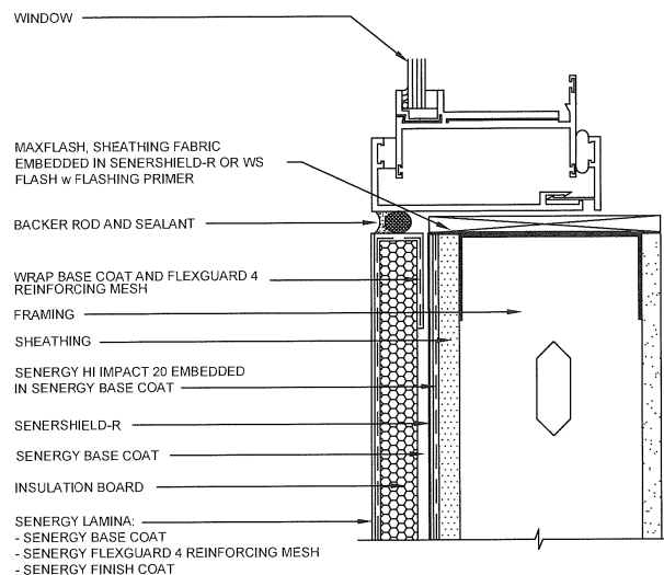
WINDOW SILL DETAIL (FLUSH)
