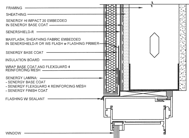
WINDOW HEAD (FLUSH)
