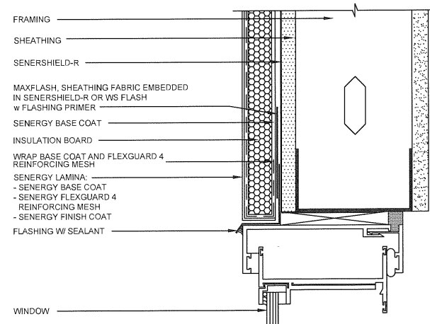
WINDOW HEAD (FLUSH)
