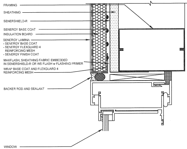
WINDOW JAMB DETAIL (FLUSH)
