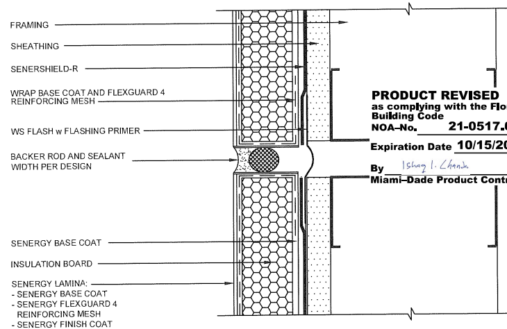
EXPANSION JOINT DETAIL (PLAN VIEW)
