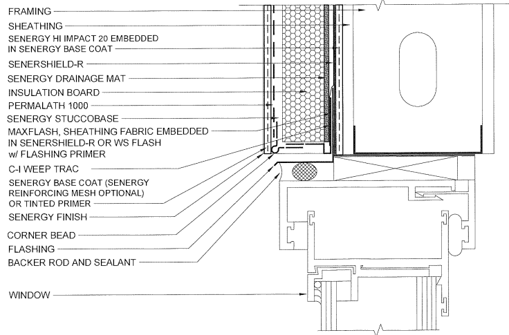
WINDOW HEAD (FLUSH)
