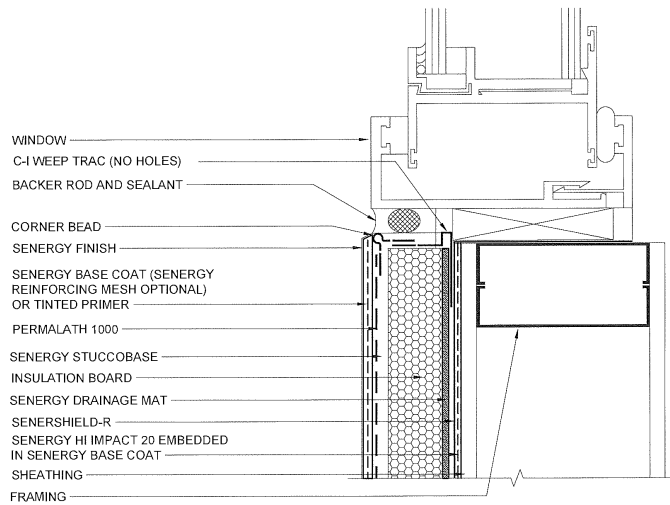
WINDOW JAMB DETAIL (FLUSH)
