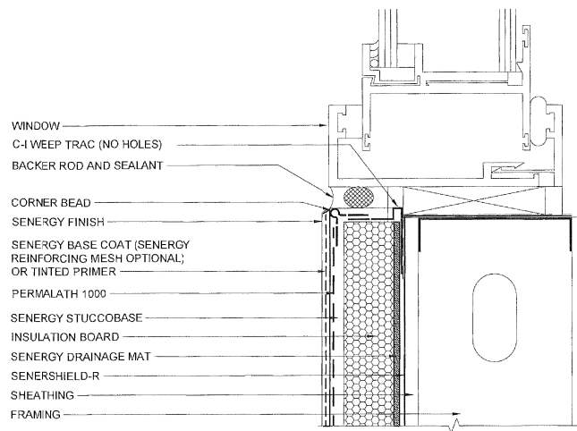
WINDOW SILL DETAIL (FLUSH)
