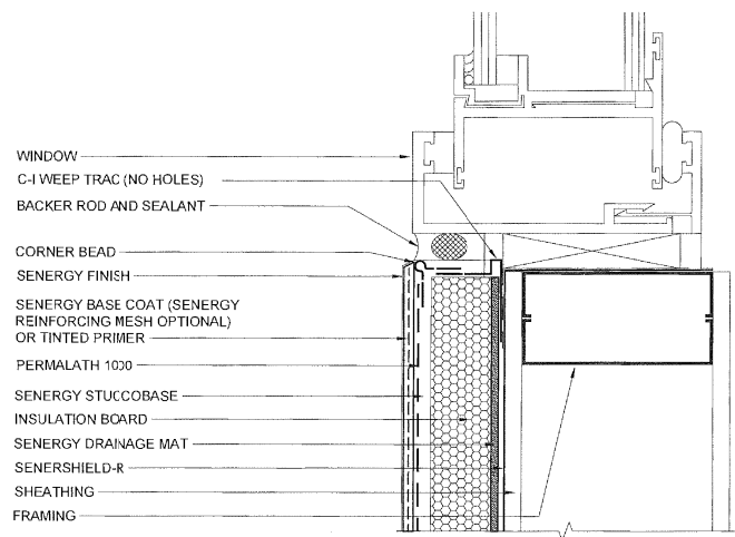
WINDOW JAMB DETAIL (FLUSH)
