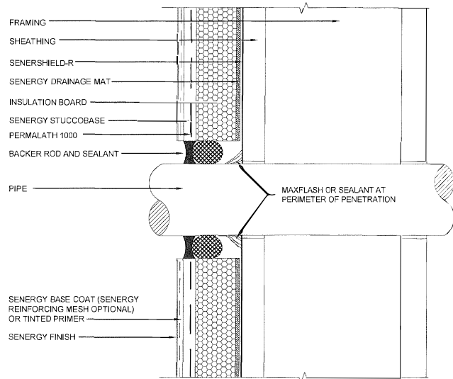
PIPE PENETRATION
