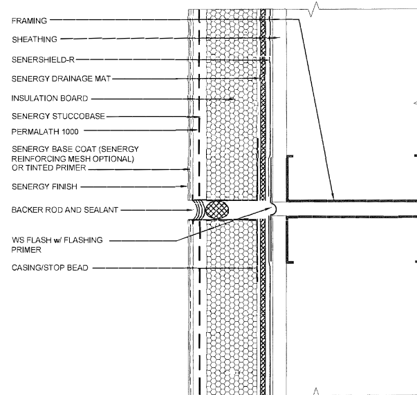
EXPANSION JOINT DETAIL (PLAN VIEW)
