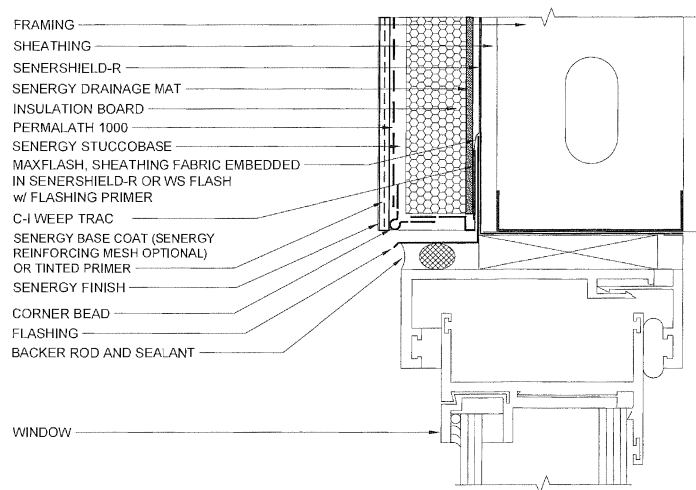
WINDOW HEAD (FLUSH)
