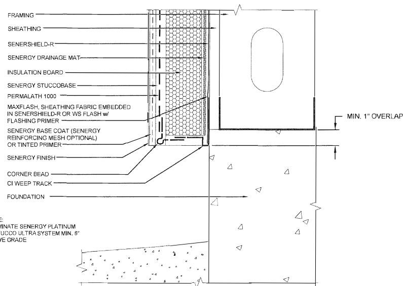
TERMINATION AT FOUNDATION
