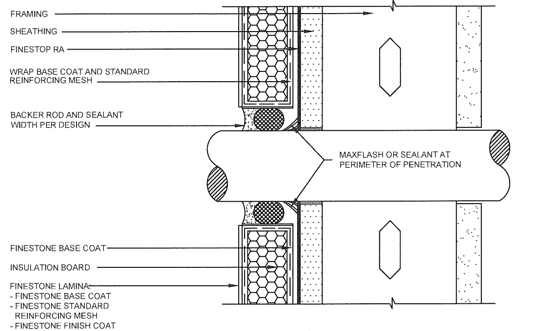
PIPE PENETRATION
