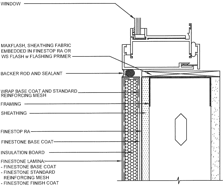
WINDOW SILL DETAIL (FLUSH)
