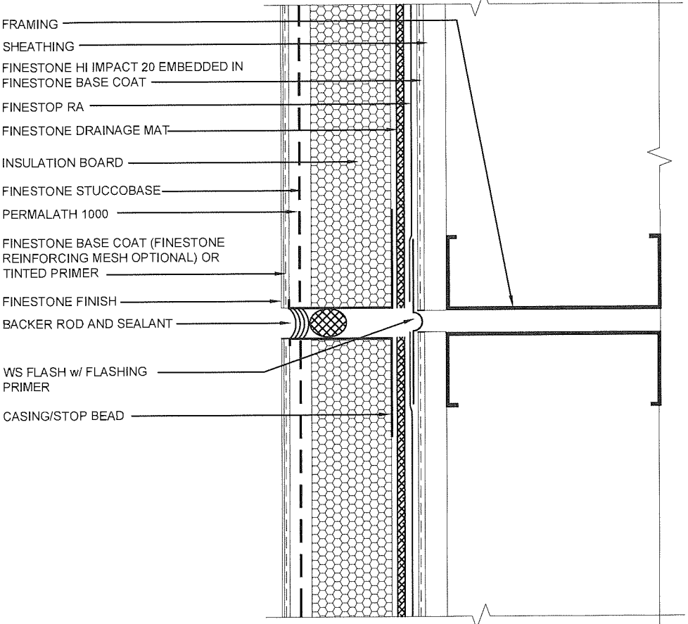
EXPANSION JOINT DETAIL (PLAN VI)
