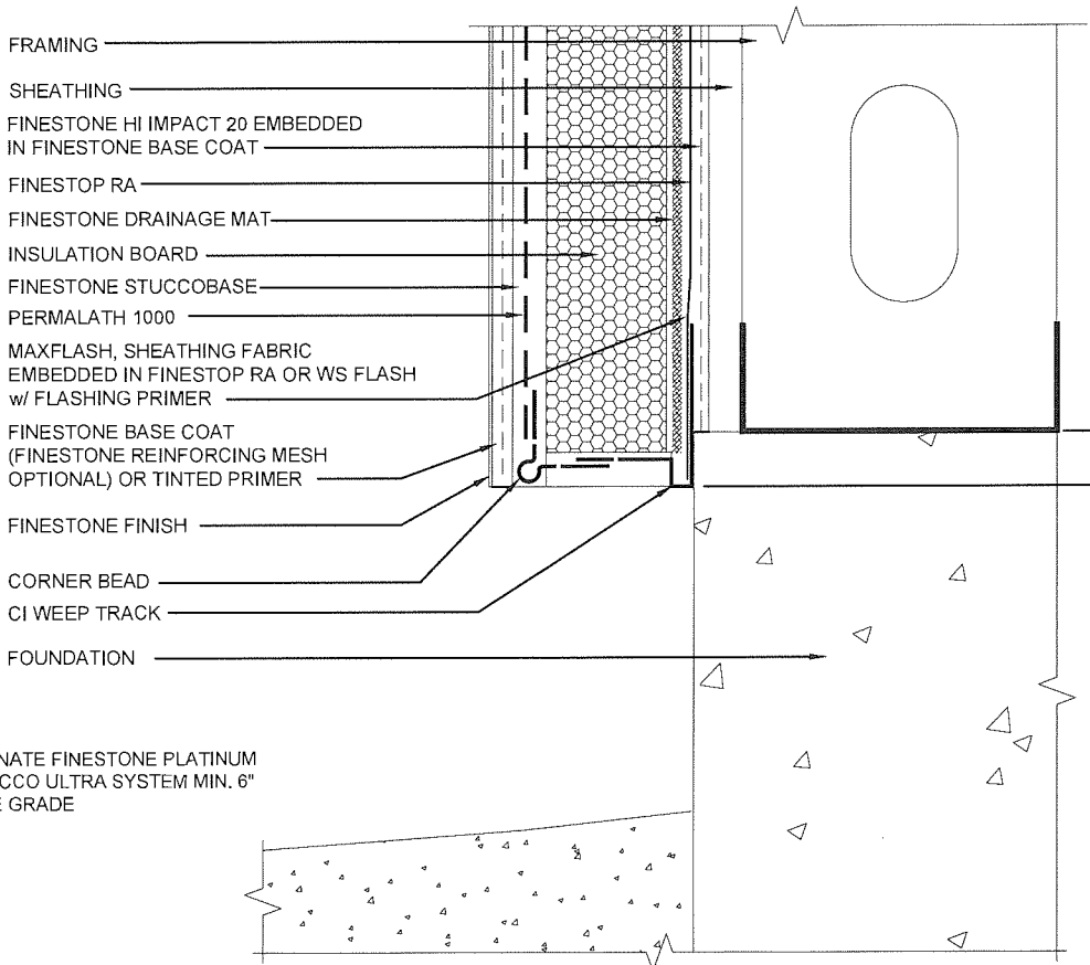
TERMINATION AT FOUNDATION
