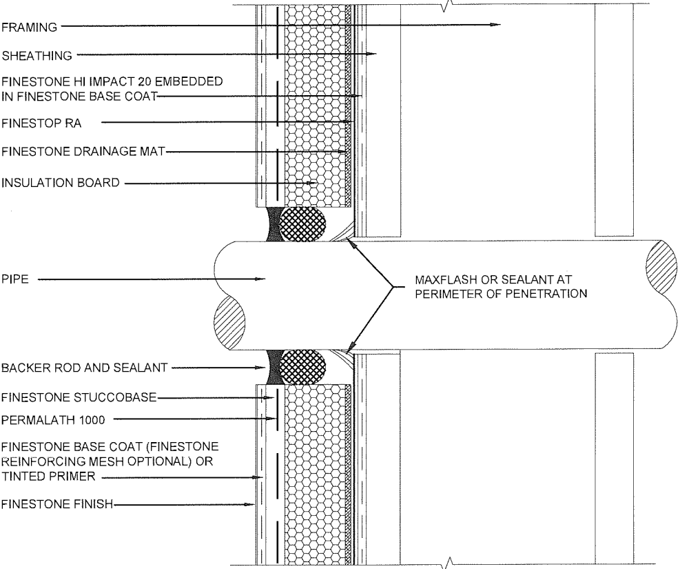
PIPE PENETRATION
