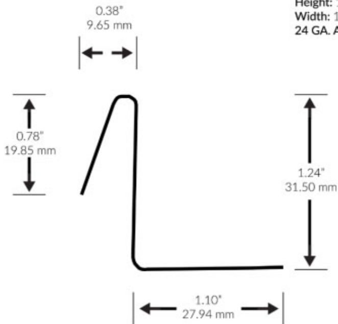
1.5" SL Continuous Clip
