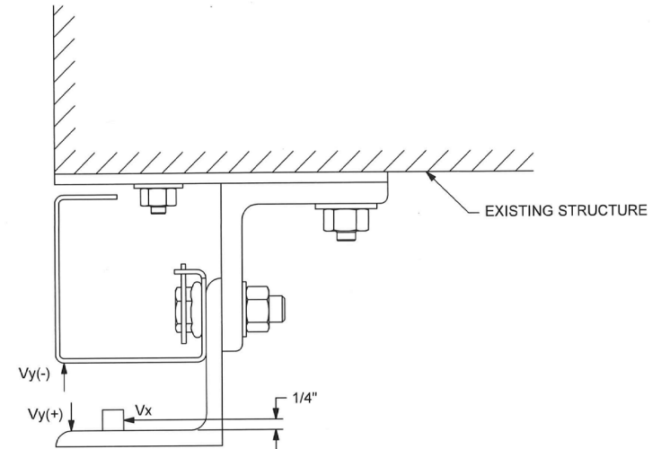
⑪ SUPERIMPOSED LOAD DIAGRAM - Z GUIDE SCALE 3/8
