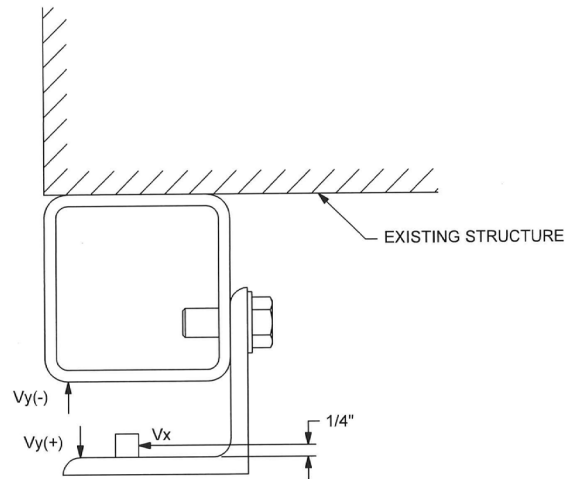
⑩ SUPERIMPOSED LOAD DIAGRAM - BOX GUIDE SCALE 3/8
