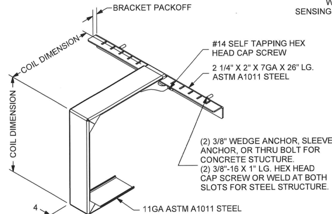
16 MID-HOOD SUPPORT (WHEN REQUIRED) SQUARE STYLE DEPICTED, "D" SHAPE ALSO AVAILABLE SCALE 3/32
