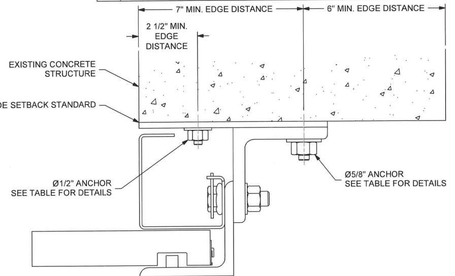
⑤ GUIDE ASSEMBLY - Z GUIDE TO CONCRETE STRUCTURE MINIMUM 4,000 PSI CONCRETE & 8\"/>
