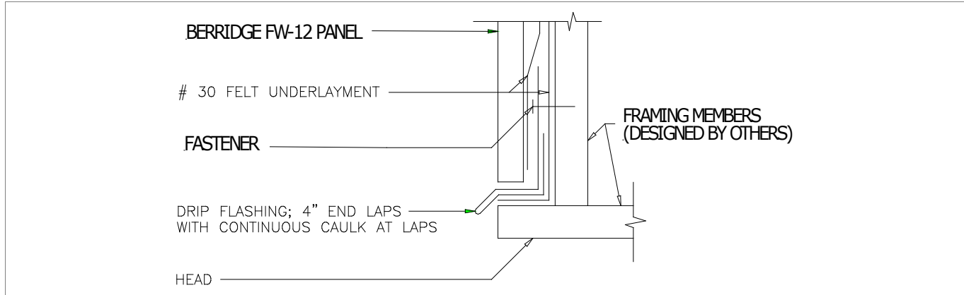
TYPICAL HEADER DETAIL
