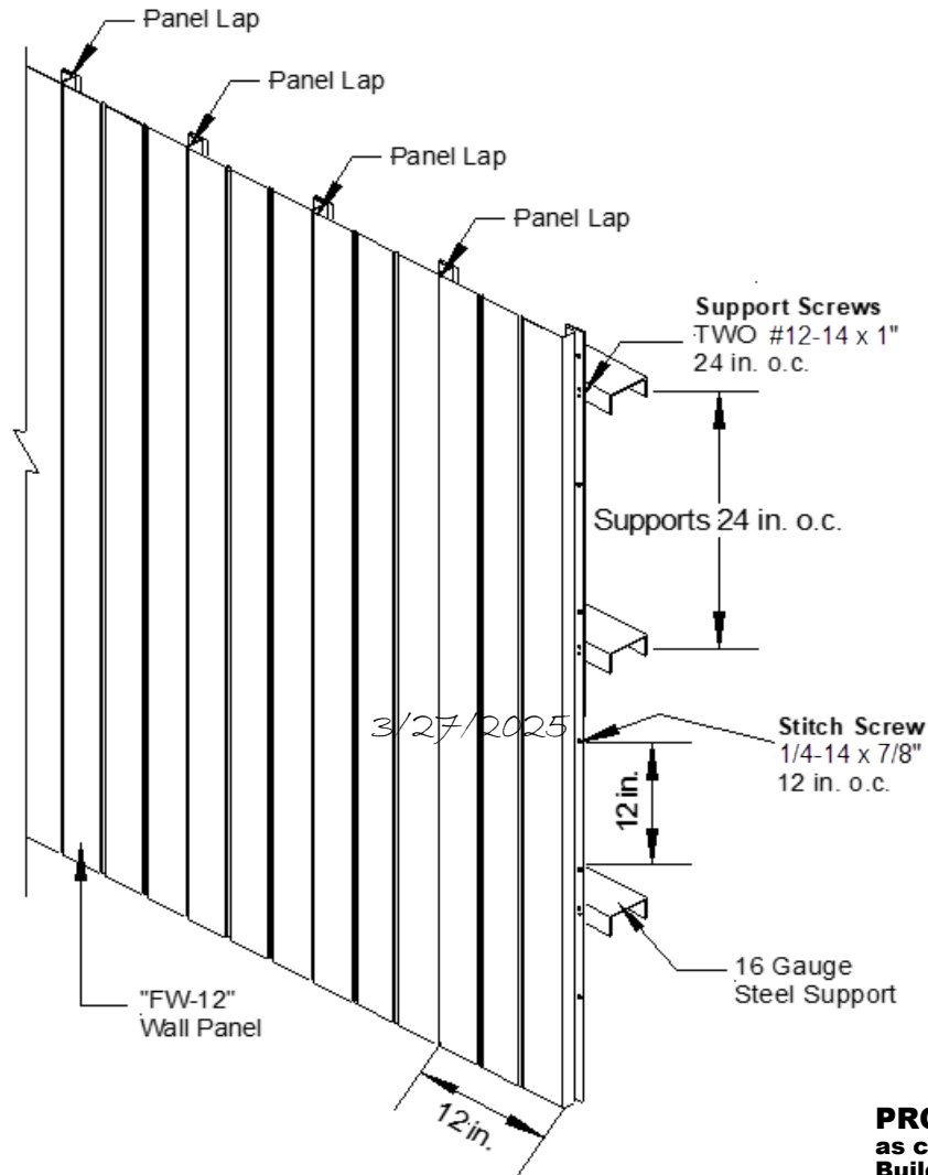
TYPICAL ELEVATION VIEW OUTSIDE OF WALL ASSEMBLY
