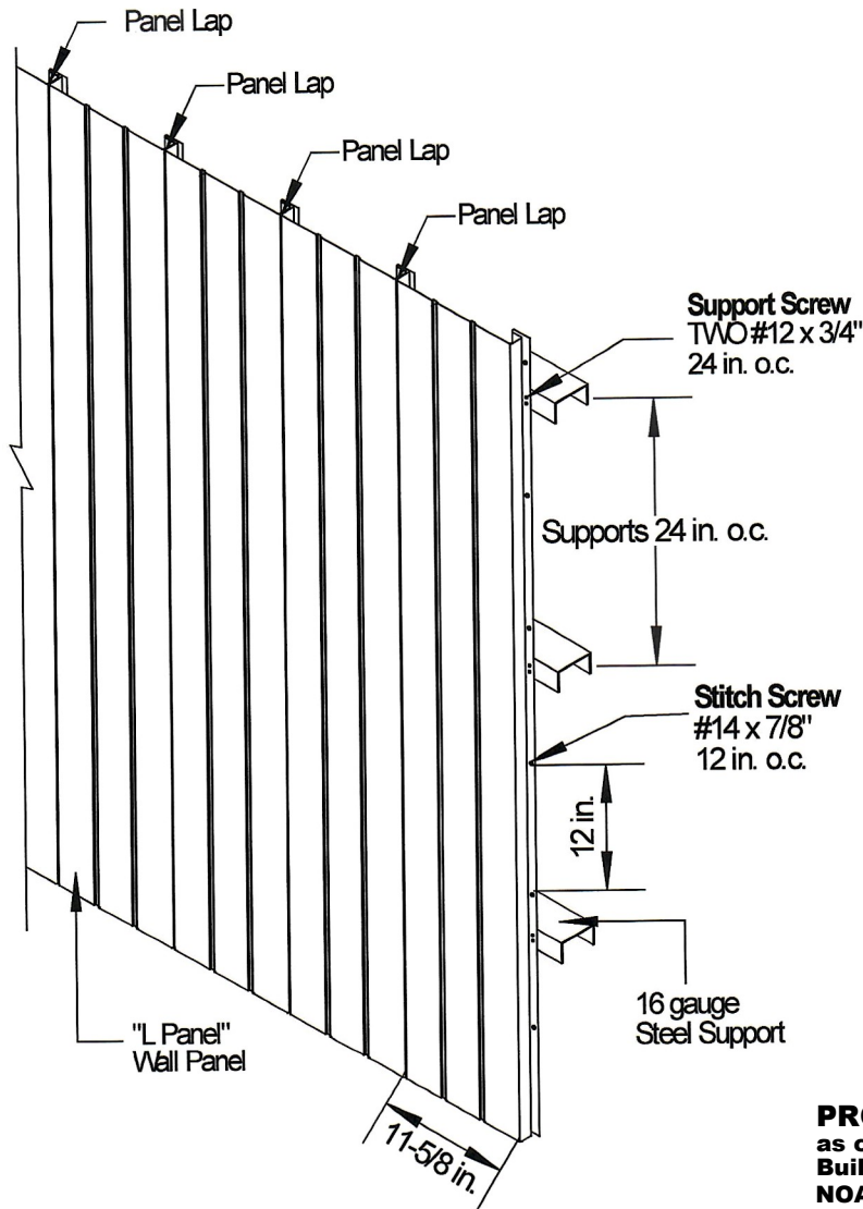
TYPICAL WALL ASSEMBLY ELEVATION VIEW
