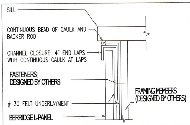
TYPICAL SILL DETAIL
