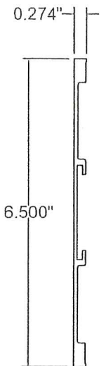
29 4" Surface Applied Muntin 6063-T6
