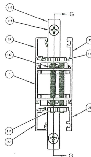
Section D-D True Divided 2" Muntin
