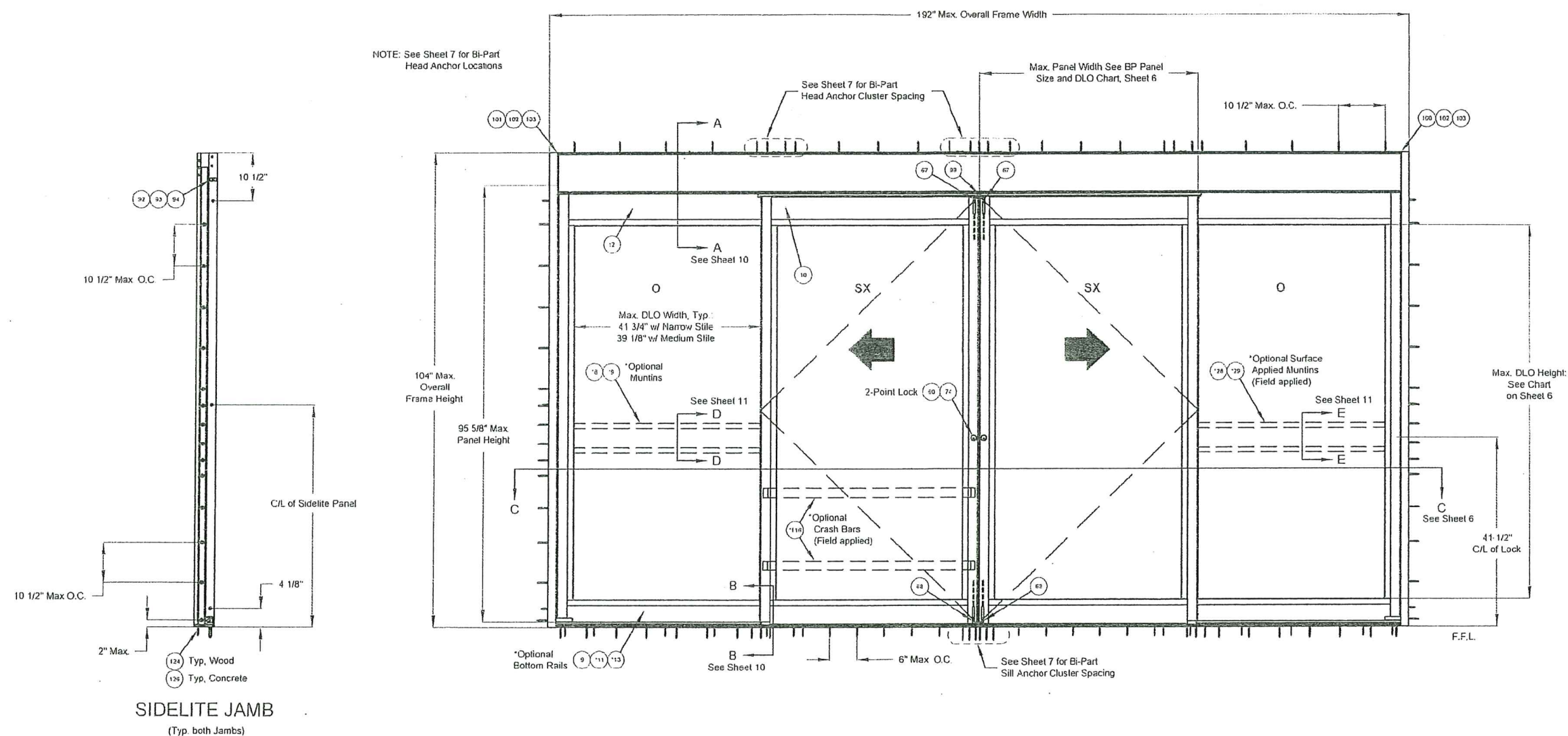
BP FSL (4 PANELS, BI-PART FIXED SIDELITE)
