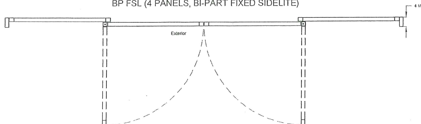
BP FSL (4 PANELS, BI-PART FIXED SIDELITE)
