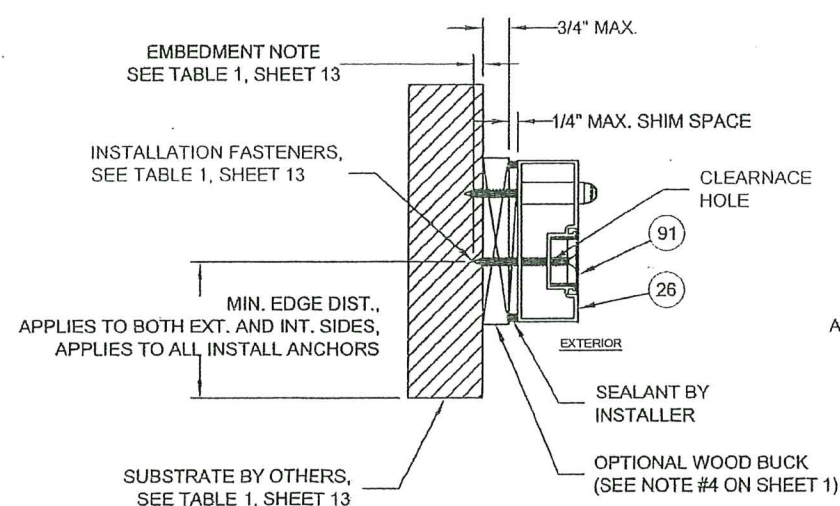
TYP. JAMB LOCK STRIKE INSTALLATION
