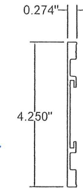
28 2" Surface Applied Muntin 6063-T6
