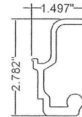
21 Resilience Track 6063-T5
