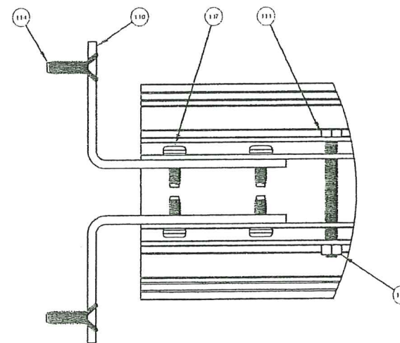
Section G-G True Divided 2" Muntin
