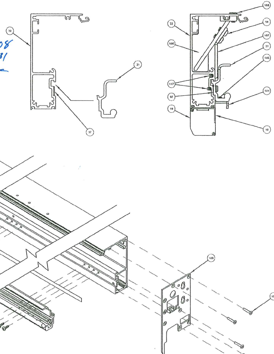
TYPICAL TRACK TO BEAM
