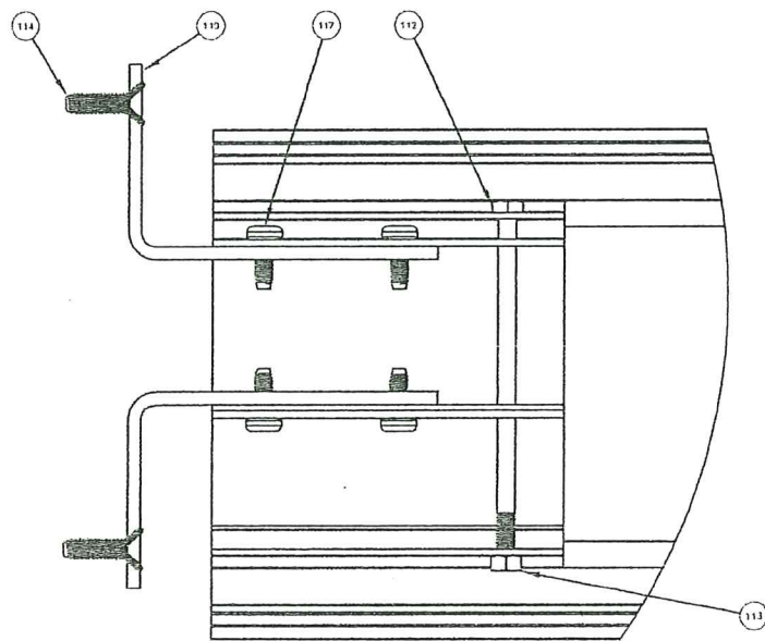
Section F-F True Divided 4" Muntin
