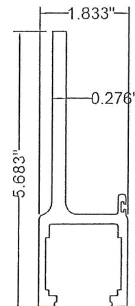
1 Carrier 6063-T6
