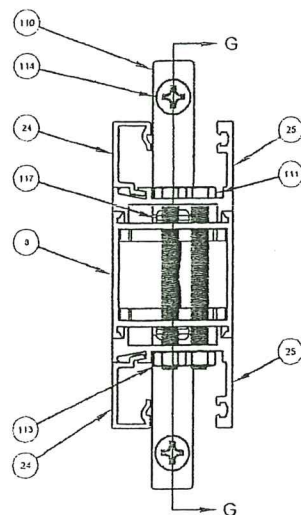
Section D-D True Divided 2" Muntin
