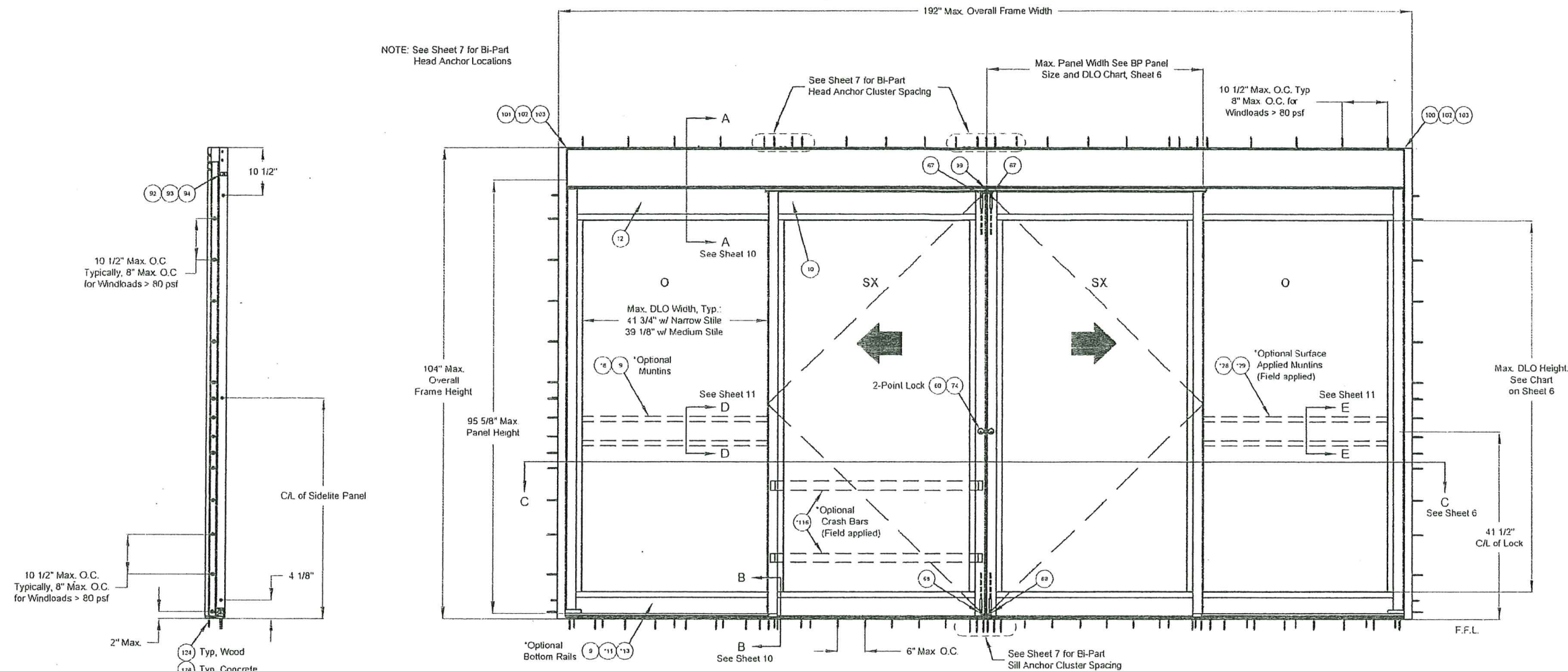
SIDELITE JAMB (Typ. both Jambs)
