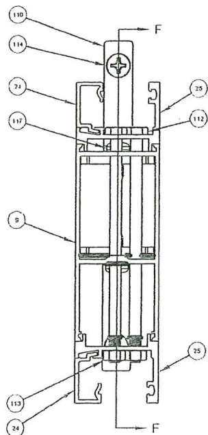
Section D-D True Divided 4" Muntin
