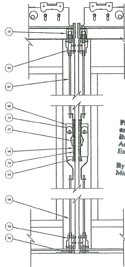
Bi-Part 4-Point Lock
