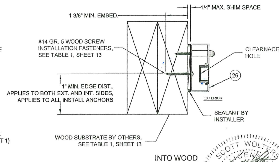
TYP. JAMB LOCK STRIKE INSTALLATION
