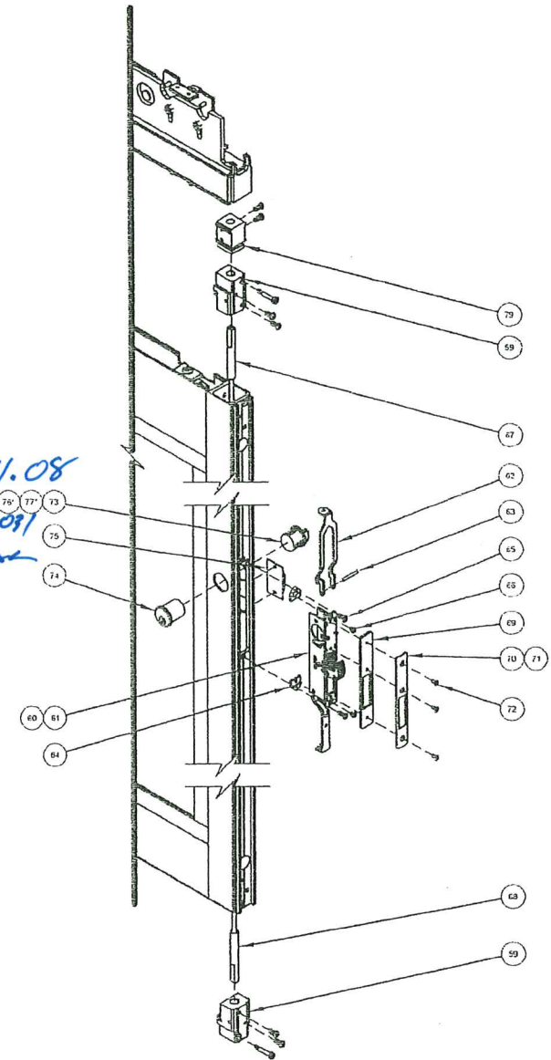
Locking System (Single Slide shown)
