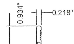
3 Sweep Housing 6063-T5
