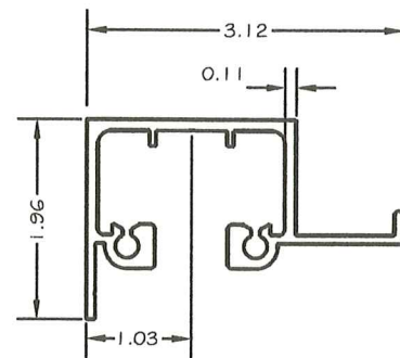
2.1- CEILING TRACK
