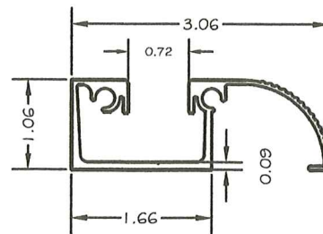
26- THRESHOLD SILL TRACK
