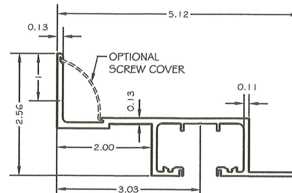
21B- 3" WALL MOUNT TRACK
