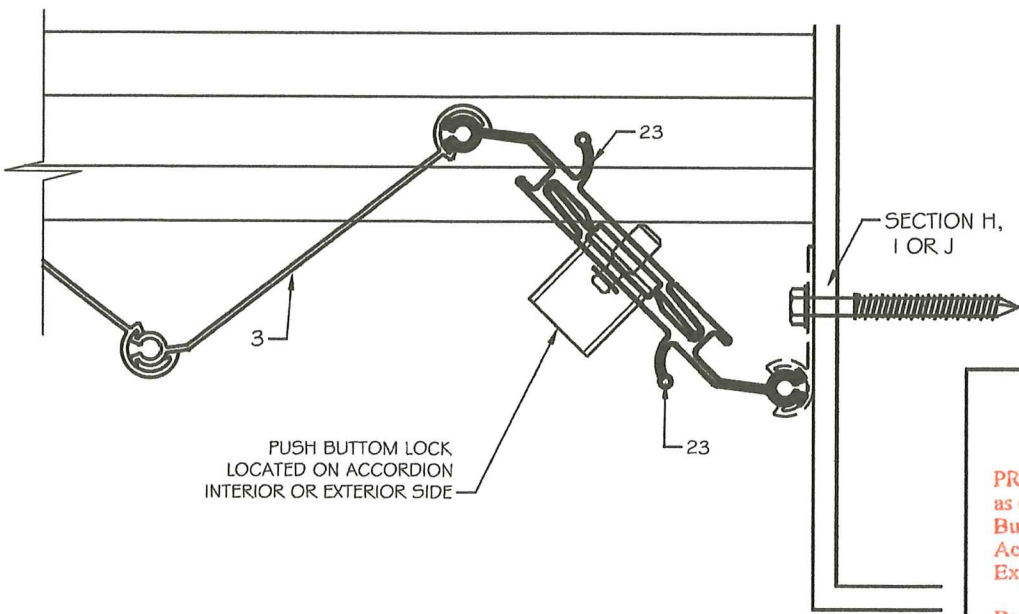
ALTERNATE SECTION L1 UNIMATE LOCK BLADE WITH STARTER BLADE SECTION
