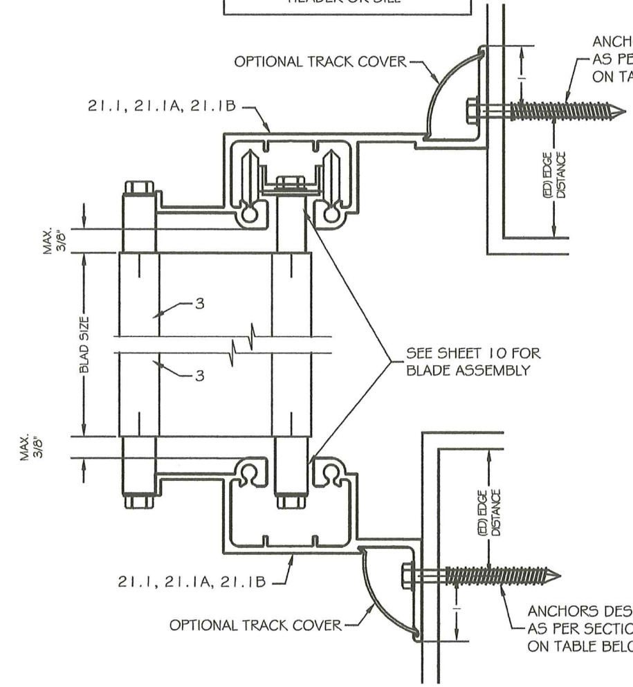
SECTION C.1.1 WALL MOUNT WITH TRACK 21.1, 21.1A OR 21.1B HEADER OR SILL
