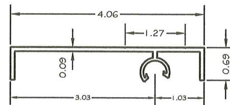
27B- 3" END CLOSURE
