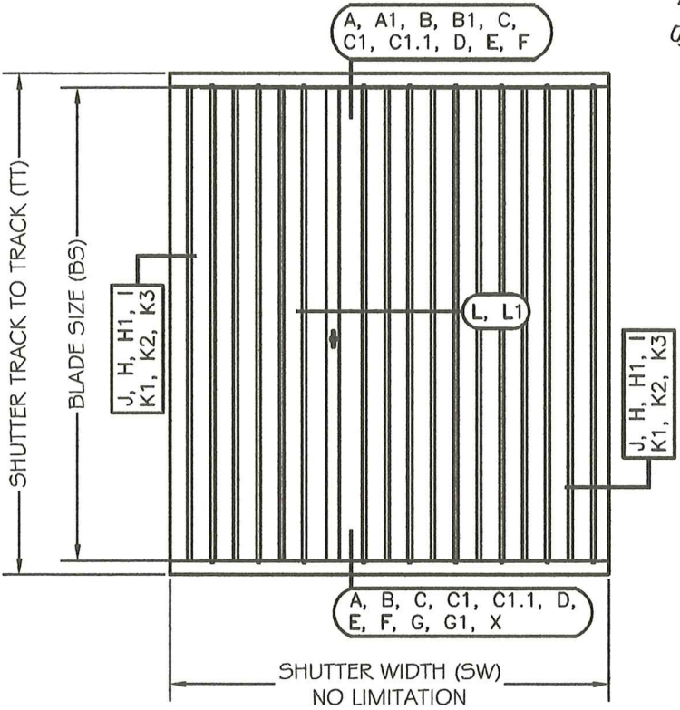
TYPICAL ELEVATION
