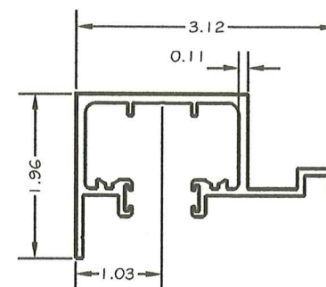
2- CEILING TRACK
