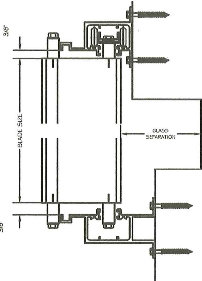
GLASS SEPARATION
