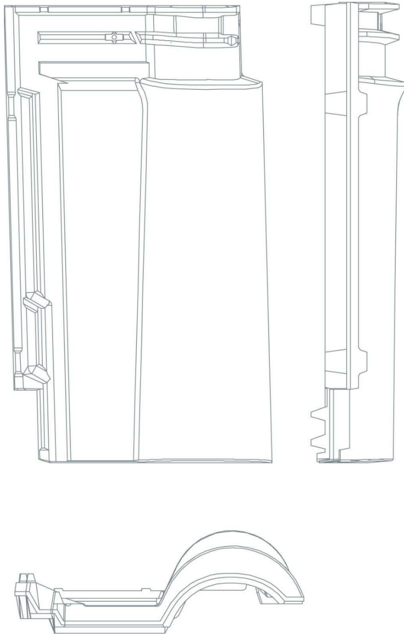
TECNO CLAY ROOF TILE
