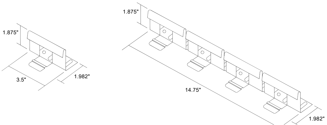
INDIVIDUAL CLIP
