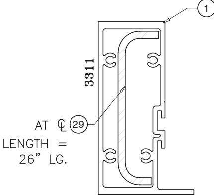
JAMB ‘J2R’ STEEL REINFORCED
