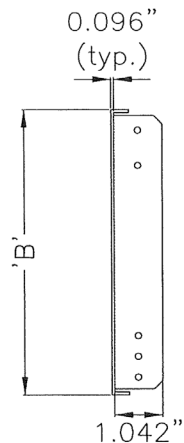
END VIEW
