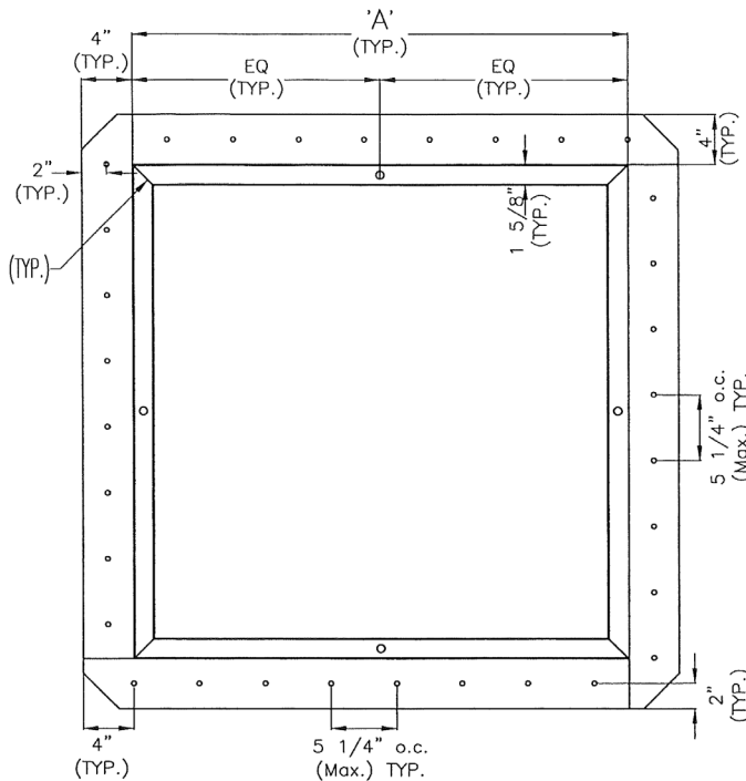
TOP VIEW
