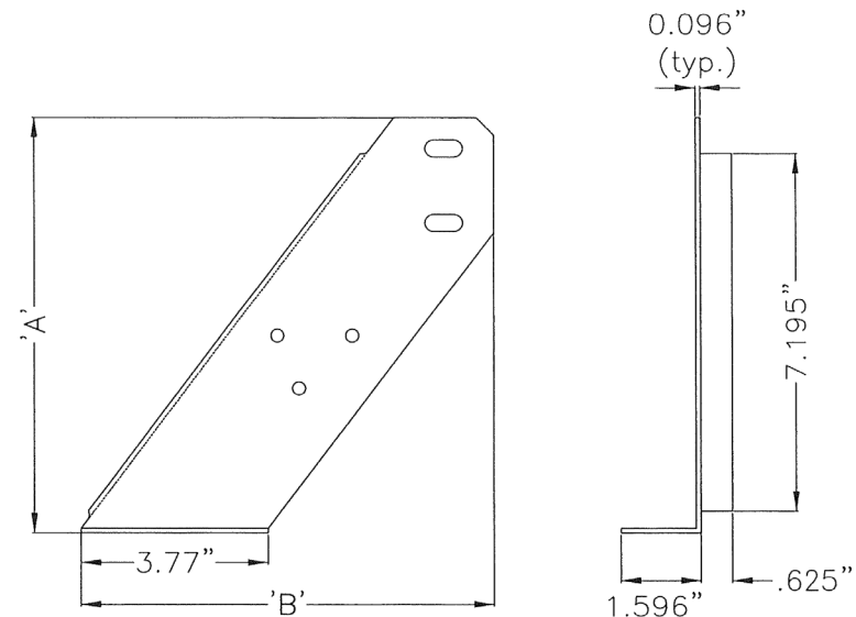
LAYOUT VIEW
