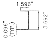
END VIEW
