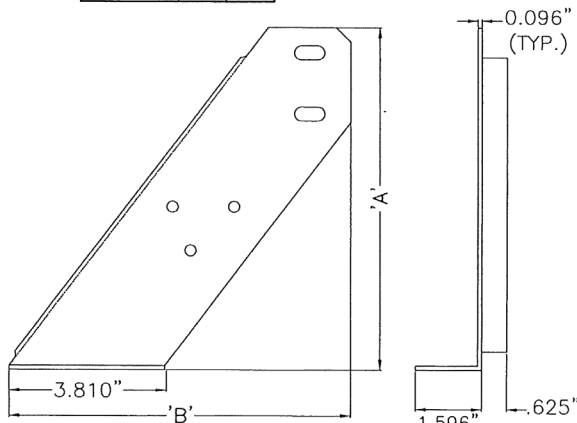
LAYOUT VIEW
