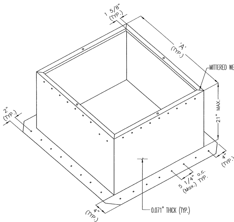
ISOMETRIC
