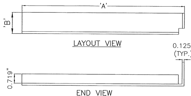
END VIEW
