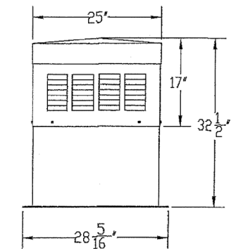
MU10 MUFFAN DIRECT DRIVE ELEVATION VIEW
