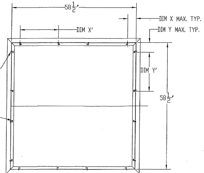
MU6020 PLAN VIEW INSTALLATION DETAILS INTERIORS COMPONENTS ARE NOT SHOWN FOR CLARITY
