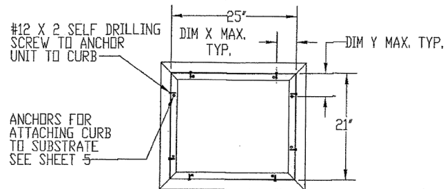
MU10 PLAN VIEW INSTALLATION DETAILS INTERIORS COMPONENTS ARE NOT SHOWN FOR CLARITY ROOF TYPE-CONCRETE
