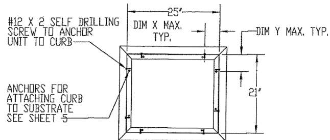
MU10 PLAN VIEW INSTALLATION DETAILS INTERIORS COMPONENTS ARE NOT SHOWN FOR CLARITY ROOF TYPE-METAL
