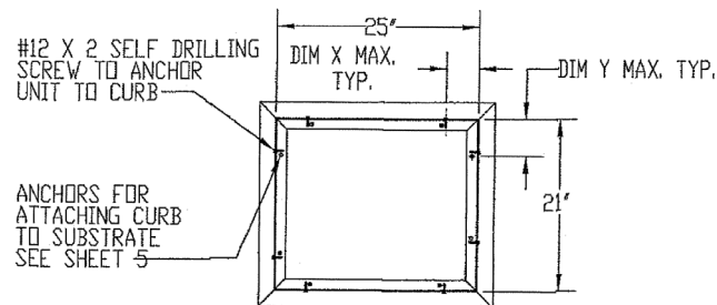
MU10 PLAN VIEW INSTALLATION DETAILS INTERIORS COMPONENTS ARE NOT SHOWN FOR CLARITY
