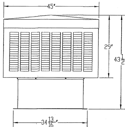
MU5018 MUFFAN BELT DRIVE ELEVATION VIEW
