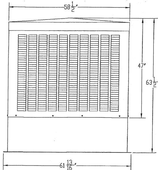
MU6020 MUFFAN BELT DRIVE ELEVATION VIEW
