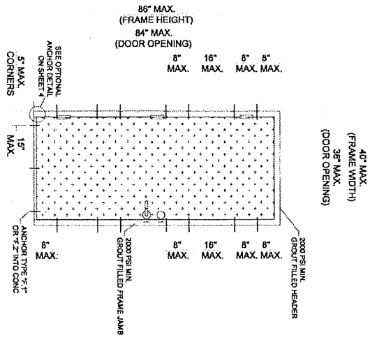
ANCHOR LAYOUT (FOR WIRE ANCHOR ONLY)
