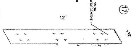
18 GA STRIKE BOX REINFORCEMENT
