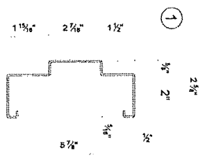
18 GA DOOR FRAME JAMB AND HEAD
