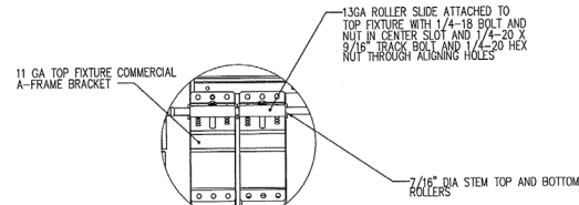
DETAIL H SCALE 1:4
