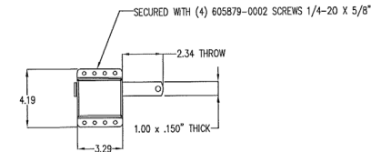
SIDE LOCK ASSY.
