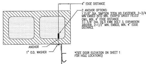
MOUNTING TO GROUT FILLED MASONRY BLOCK DETAIL
