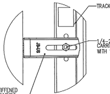
TYPICAL TRACK AND JAMB FASTENERS DETAIL
