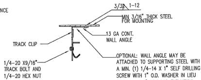
MOUNTING TO STEEL JAMB DETAIL
