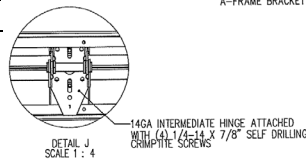
DETAIL J SCALE 1:4
