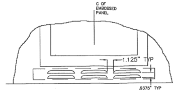
VENT DETAILS
