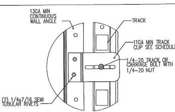
TYPICAL TRACK CLIP RIVETING DETAIL
