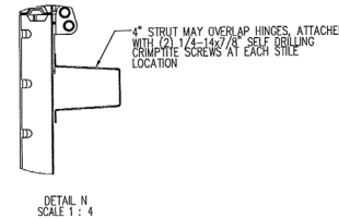
DETAIL N SCALE 1 : 4
