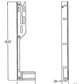
FLAG ANGLE 13GA
