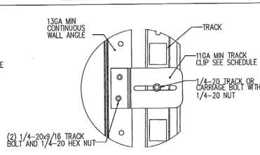
TYPICAL TRACK CLIP BOLTING DETAIL
