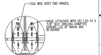
DETAIL I SCALE 1:4
