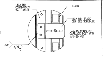
TYPICAL TRACK CLIP WELDING DETAIL
