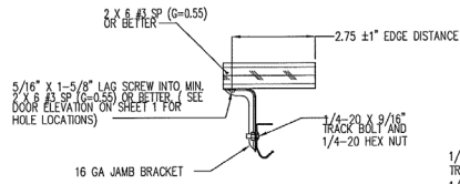
MOUNTING TO WOOD JAMB DETAIL
