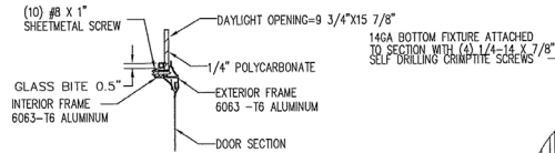
WINDOW DETAIL SECTION F-F SCALE 1:4
