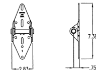
#1 END HINGE / CENTER HINGES 14GA
