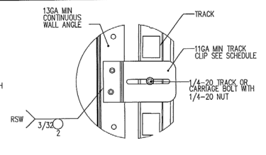
TYPICAL TRACK CLIP WELDING DETAIL
