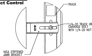
TYPICAL TRACK AND JAMB FASTENERS DETAIL
