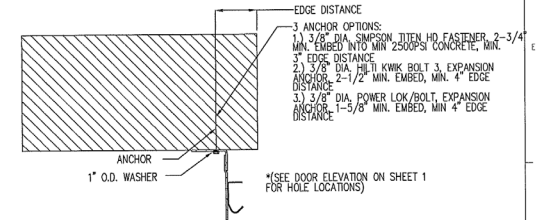
MOUNTING TO 2500PSI CONCRETE DETAIL
