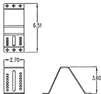
BASE TOP FIXTURE 11GA
