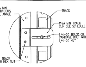
TYPICAL TRACK CLIP BOLTING DETAIL
