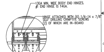
DETAIL K SCALE 1 : 4
