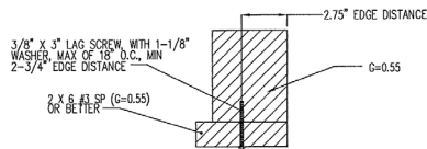
WOOD MOUNTED TO #3 SOUTHERN PINE SUBSTRATE
