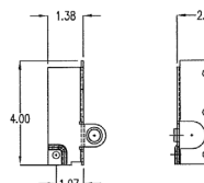
BOTTOM FIXTURE 14 GA
