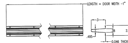
3" STRUT OPEN W/ (UBAR) 80 KSI MIN. YIELD STRENGTH, 3" X 18GA
