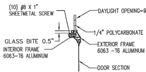
WINDOW DETAIL
