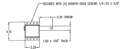
SIDE LOCK ASSY.
