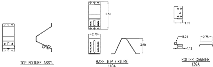
TOP FIXTURE DETAILS
