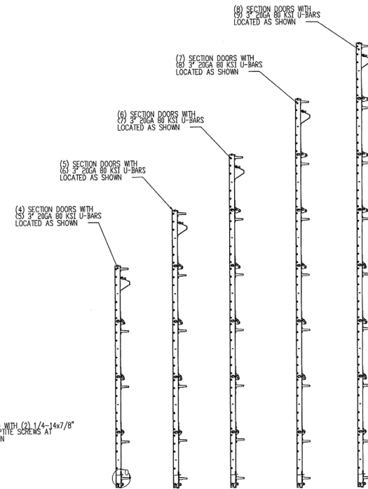
STRUT LOCATIONS SCALE 1 : 16
