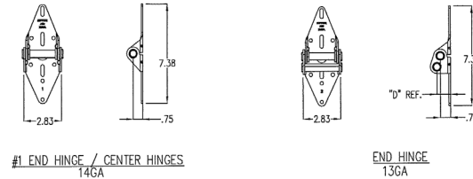
HINGE DETAILS
