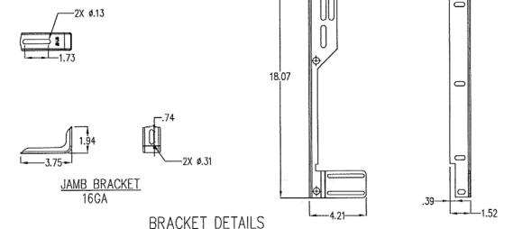
BRACKET DETAILS
