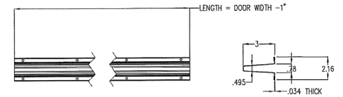
STRUT DETAILS
