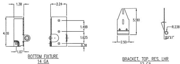
BOTTOM FIXTURE DETAILS
