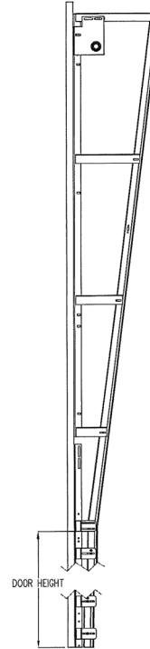
VERTICAL LIFT TRACK DETAIL
