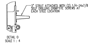
DETAIL O SCALE 1 : 4
