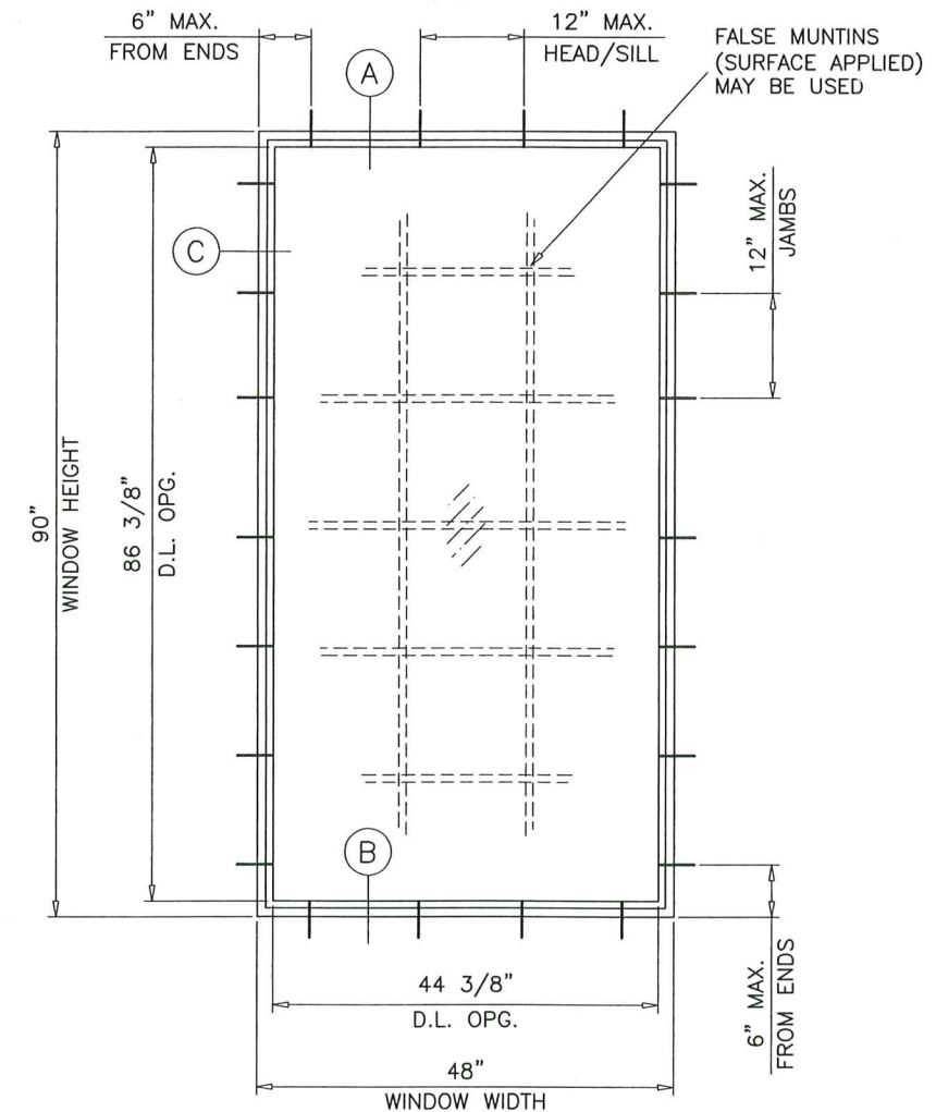
TYPICAL ELEVATION
