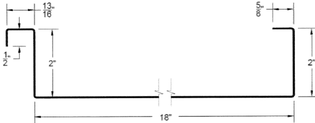
PAC-2400 – 24GA. (MIN.) STEEL PANEL (18" WIDE)
