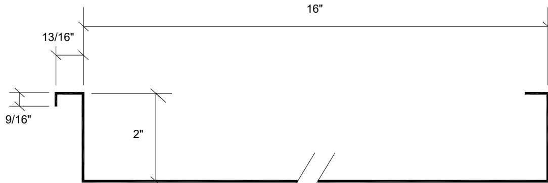
PAC-2400 – 24GA. (MIN.) STEEL PANEL (16" WIDE)
