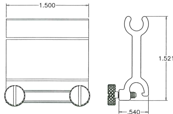
SA-EXTENDED TRACK CLAMP SCALE 1:1
