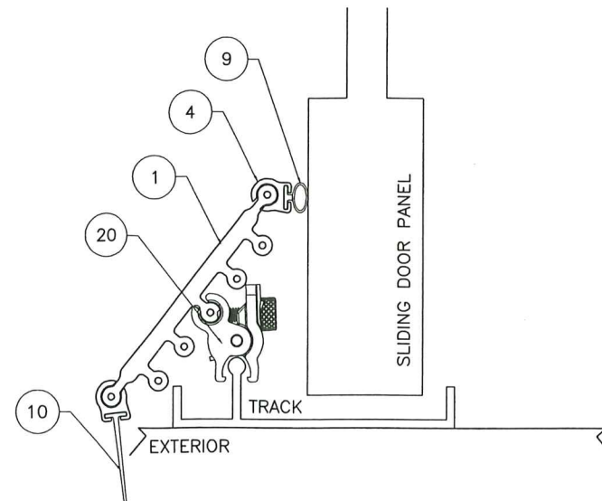
EXTERIOR MECHANICAL ATTACHMENT WITH SPRING LOADED TRACK CLAMP
