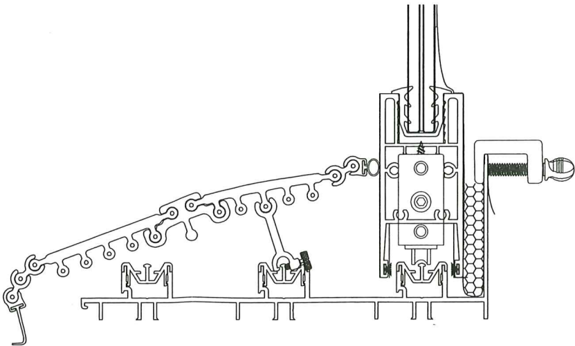
INSTALLATION (THRESHOLD/SILL RISER) (EXAMPLE) ES-6600
