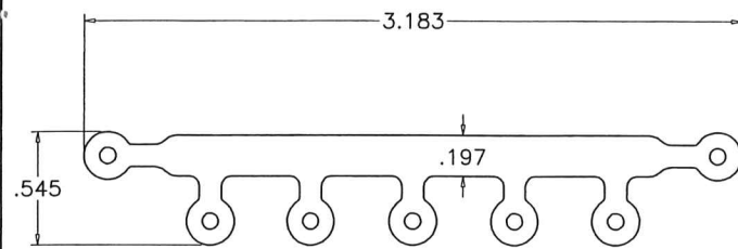
SA-SHIELD SCALE 1:1
