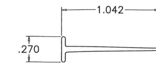
SA-FLAP SEAL
