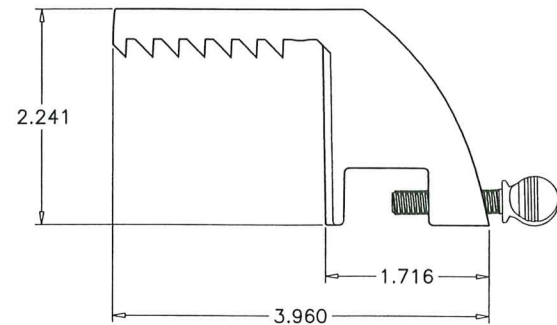
LARGE TRACK CLAMP SCALE 1:2
