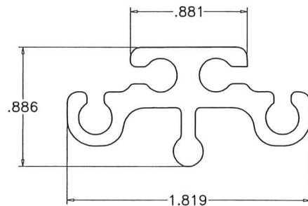
SA-LINK SCALE 1:1
