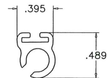
WEATHERSTRIP ADAPTER SCALE 1:1
