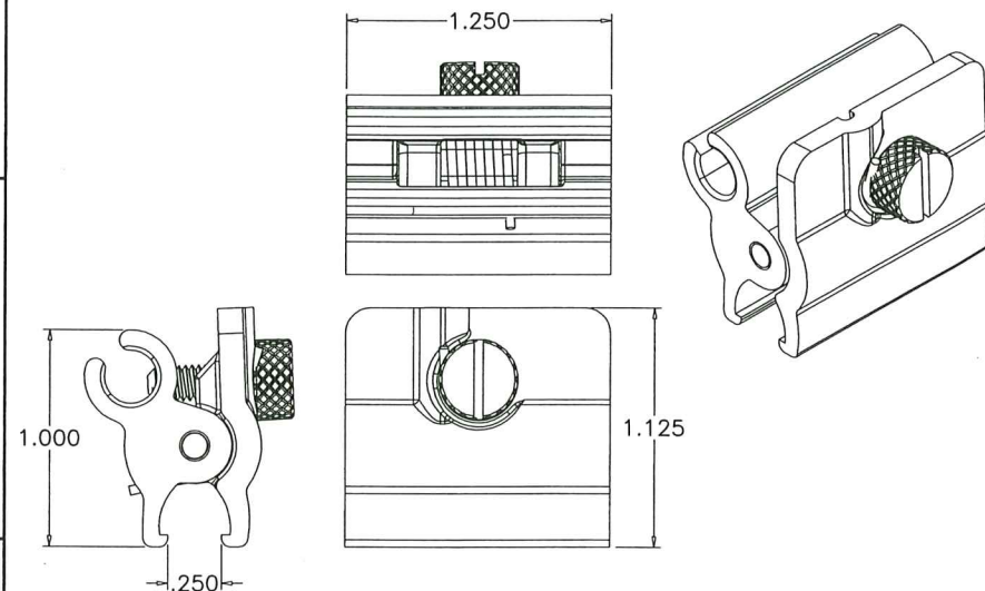
SA-EXTENDED TRACK CLAMP SCALE 1:1
