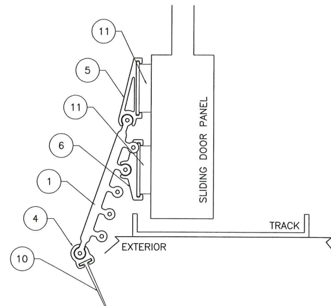
EXTERIOR ADHESIVE ATTACHMENTS
