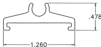
SA-6 IN. ADHESIVE SEAL BASE SCALE 1:1
