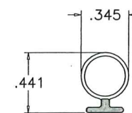
SA-BULB SEAL
