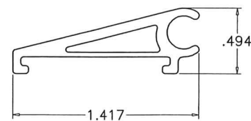
SA-ADHESIVE SEAL BASE SCALE 1:1
