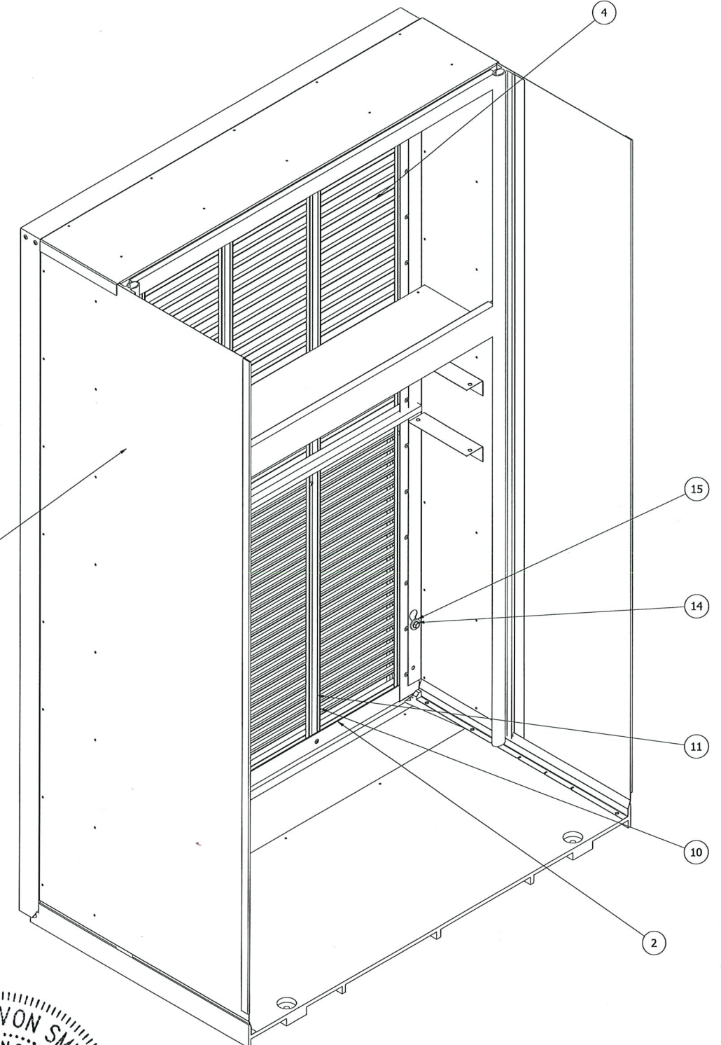
WALL SLEEVE ATTACHMENT DETAIL REAR VIEW N.T.S.
