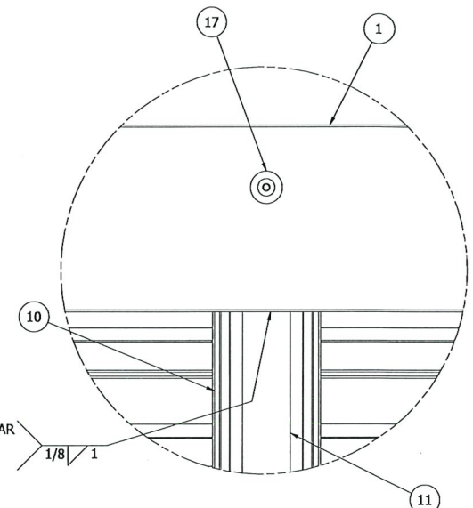
7 BRACE BAR WELDMENT CONSTRUCTION DETAILS 2,3,4 N.T.S.
