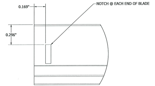
DETAIL AD
