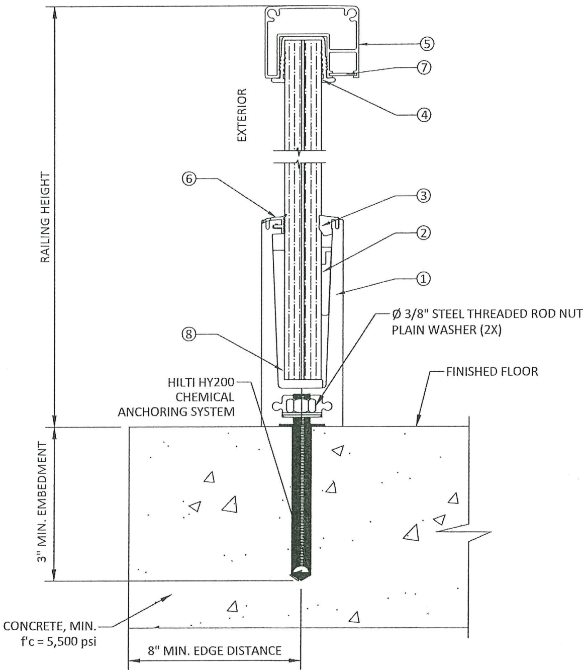
ANCHOR OPTION #1
