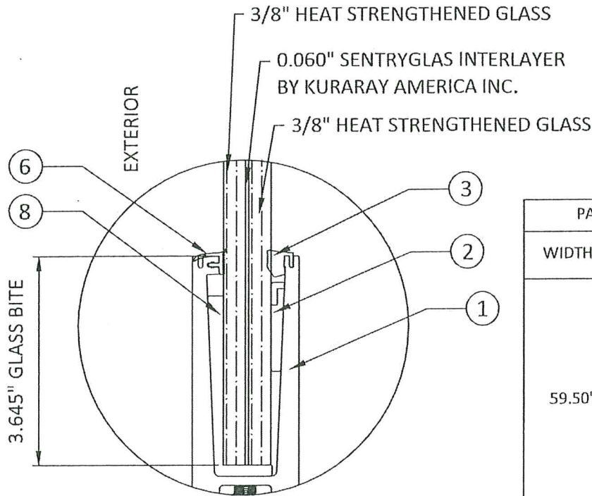
GLAZING DETAIL
