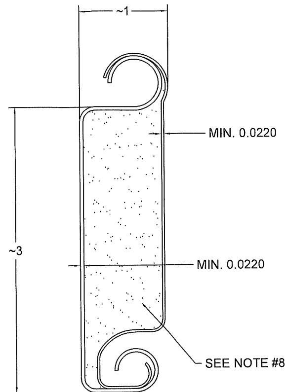
③ TYPICAL SECTION SLAT DETAIL
