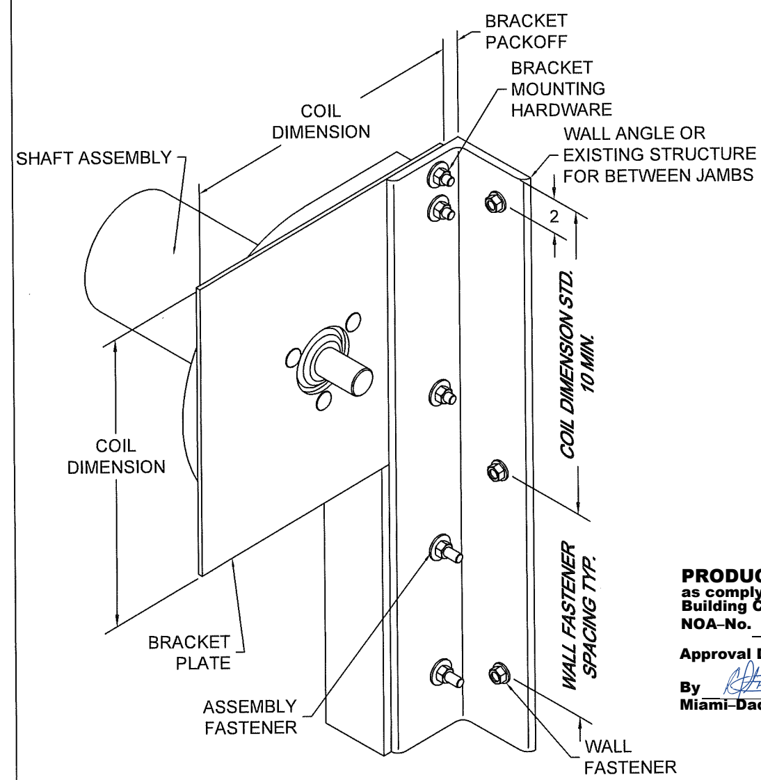
16 BRACKET MOUNTING / TOP WALL ANGLE FASTENING BRACKET MOUNTING PER DETAIL 8 DEPICTED, OTHER BRACKET MOUNTINGS ARE AVAILABLE SCALE: NTS
