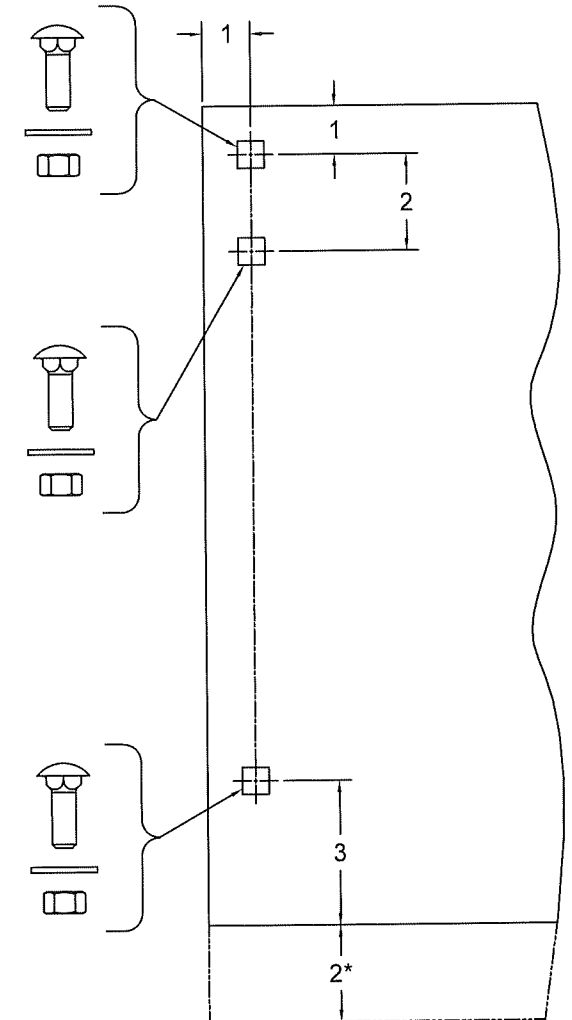
⑧ BRACKET MOUNTING DETAIL 0.172 MIN. THICKNESS * 2" EXTENSION WHEN 8" AND LARGER SHAFT ASSEMBLY IS SUPPLIED 1/4 SCALE
