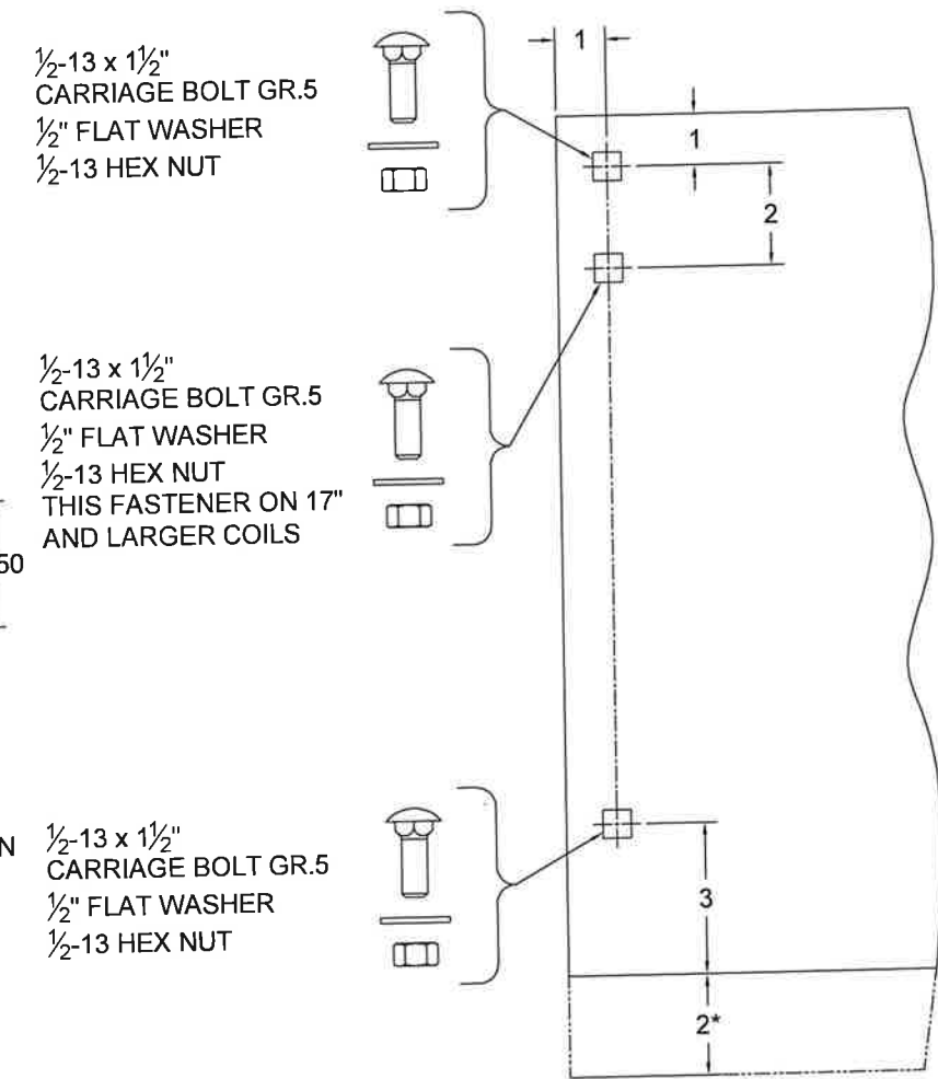
⑧ BRACKET MOUNTING DETAIL 0.172 MIN. THICKNESS
