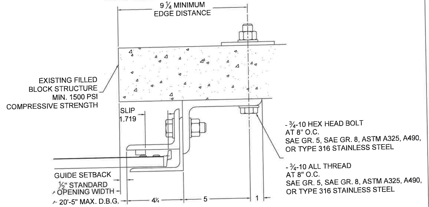
① GUIDE ASSEMBLY FILLED BLOCK STRUCTURE (Z-GUIDE)
