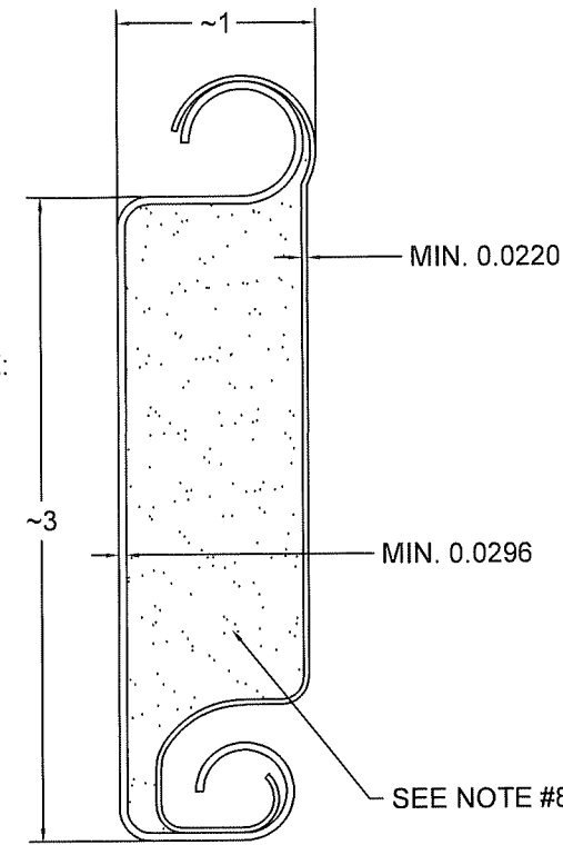
③ SLAT DETAIL TYPICAL SECTION
