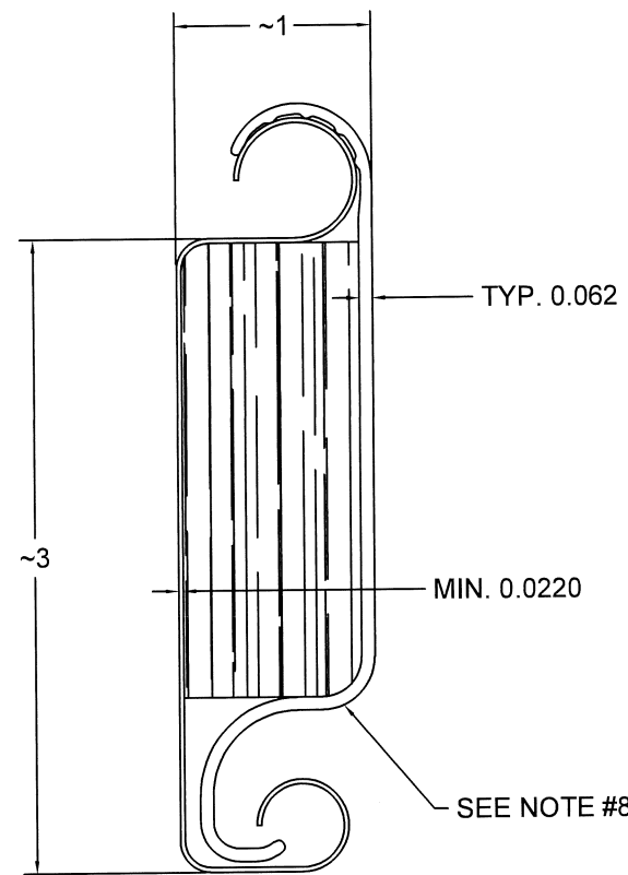
③ SLAT DETAIL TYPICAL SECTION FRONT SLAT:
