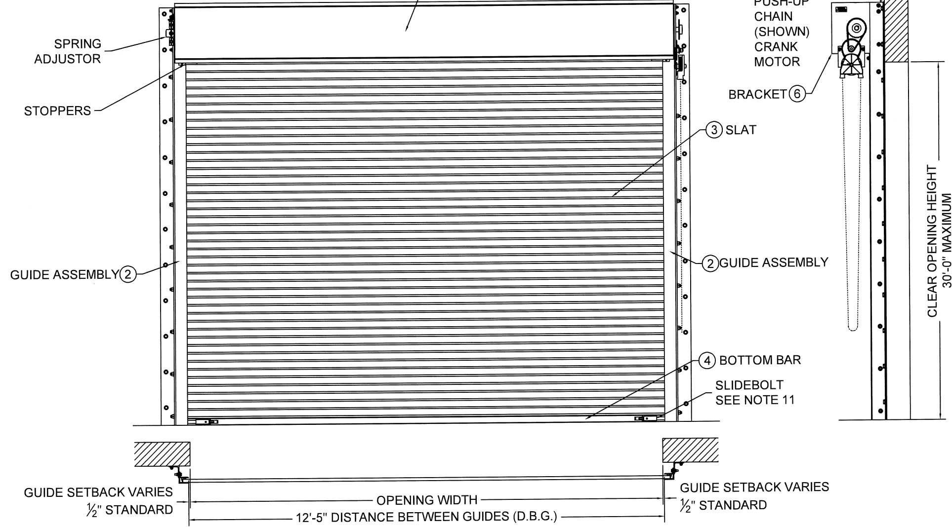
① OVERALL DOOR ASSEMBLY 1:32 SCALE
